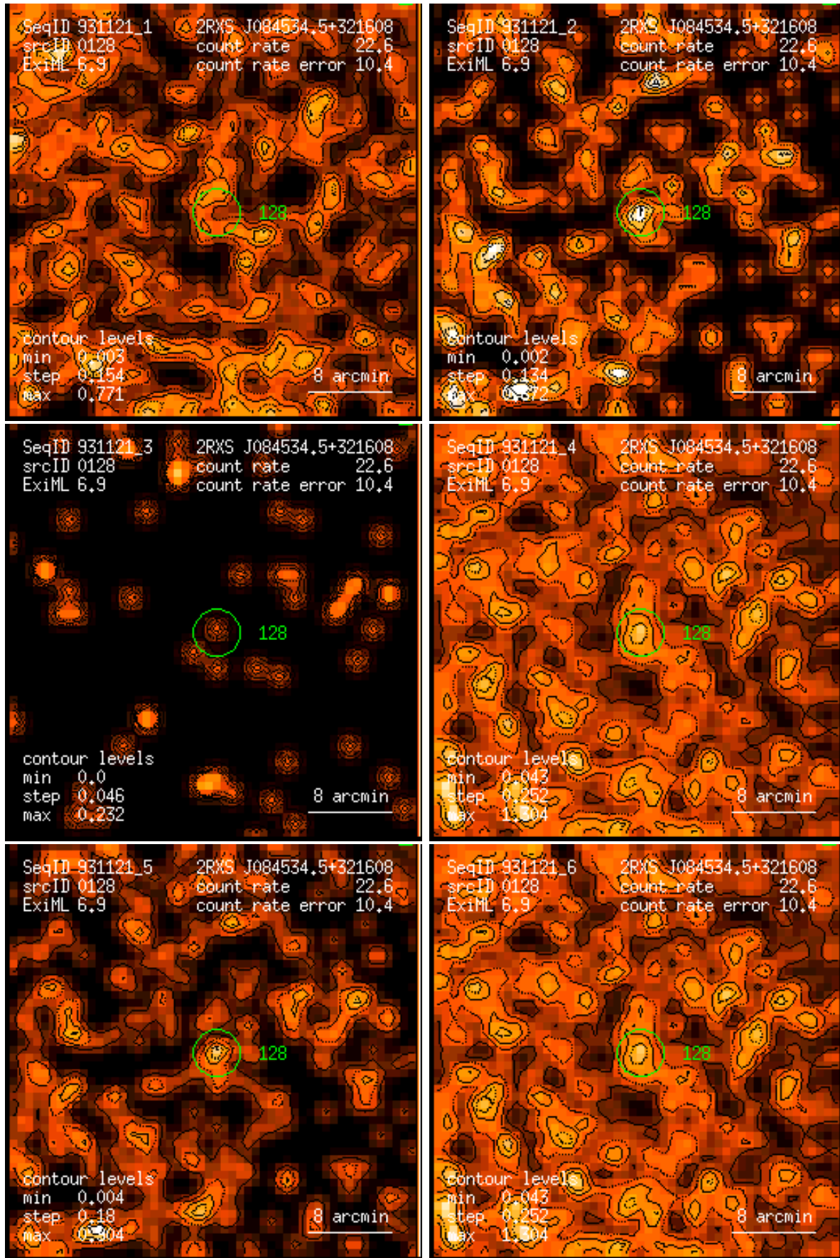
Figure 128: RASS 931121: detection 0128: band rate images, Gaussian filter: (1) PSPC channels 11 – 41, (2) 52 – 90, (3) 91 – 201, (4) 11 – 235, (5) 52 – 201, (6) 11 – 201. Broad band rates in counts/ks. Band rate contour levels in counts/ks/arcmin 2 .
