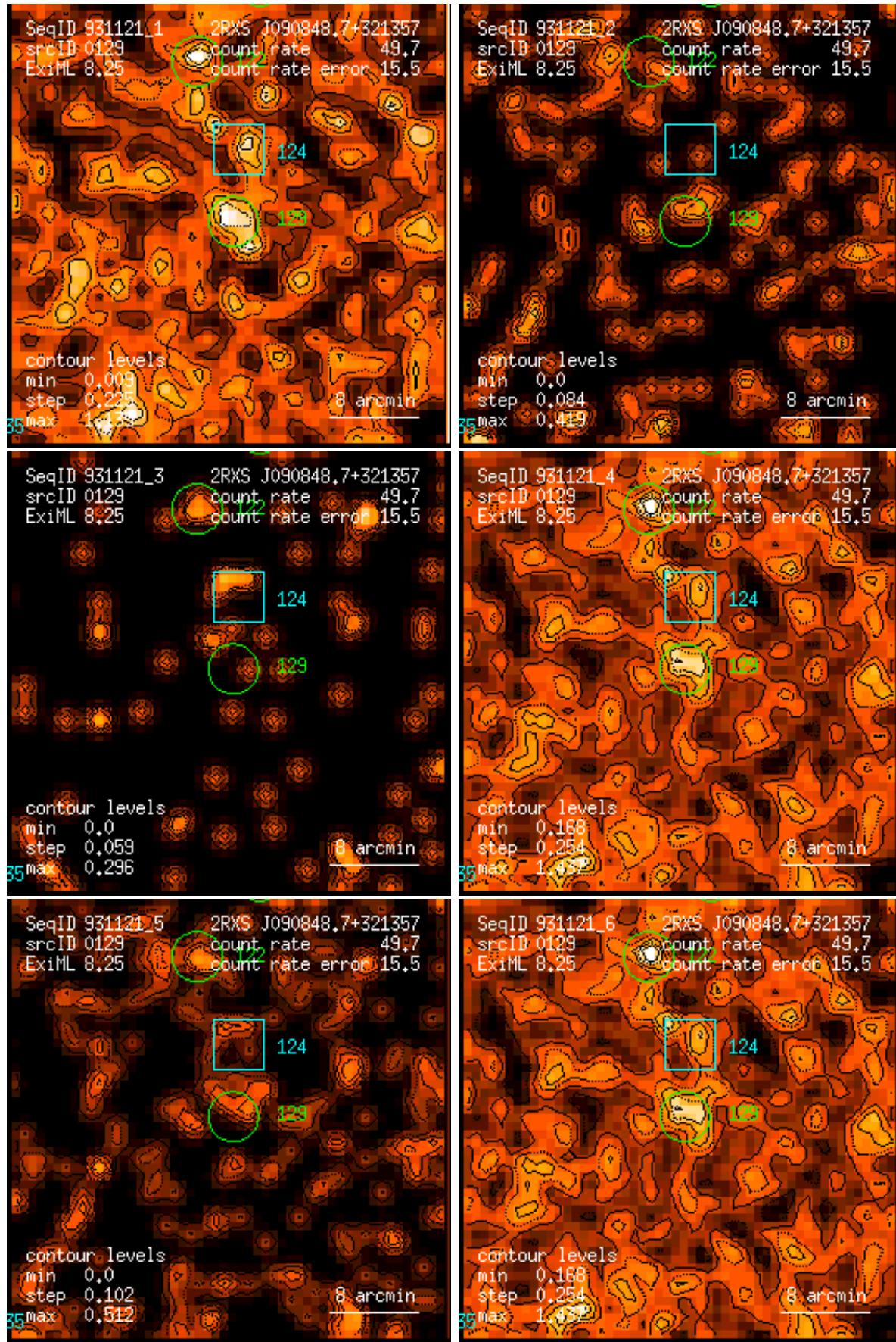
Figure 129: RASS 931121: detection 0129: band rate images, Gaussian filter: (1) PSPC channels 11 – 41, (2) 52 – 90, (3) 91 – 201, (4) 11 – 235, (5) 52 – 201, (6) 11 – 201. Broad band rates in counts/ks. Band rate contour levels in counts/ks/arcmin 2 .
