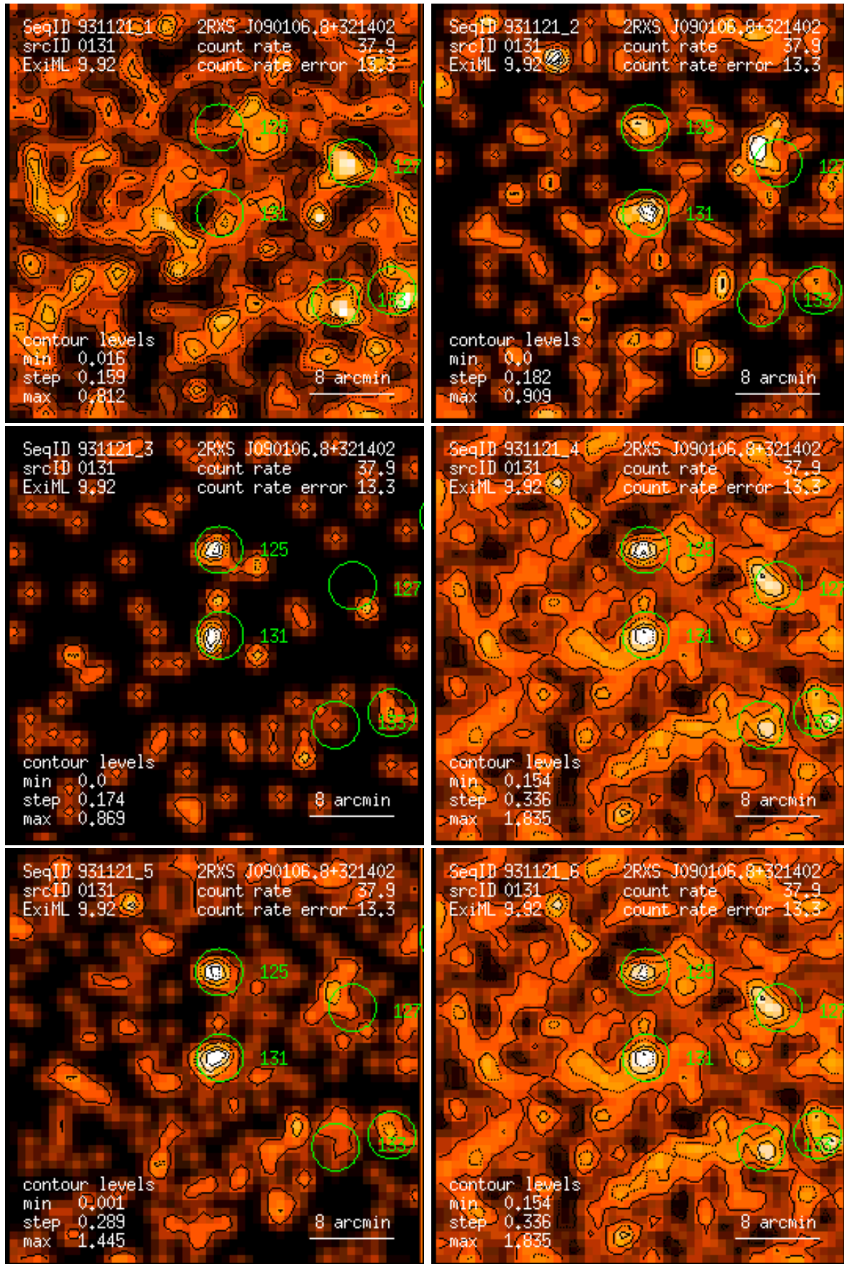
Figure 131: RASS 931121: detection 0131: band rate images, Gaussian filter: (1) PSPC channels 11 – 41, (2) 52 – 90, (3) 91 – 201, (4) 11 – 235, (5) 52 – 201, (6) 11 – 201. Broad band rates in counts/ks. Band rate contour levels in counts/ks/arcmin 2 .
