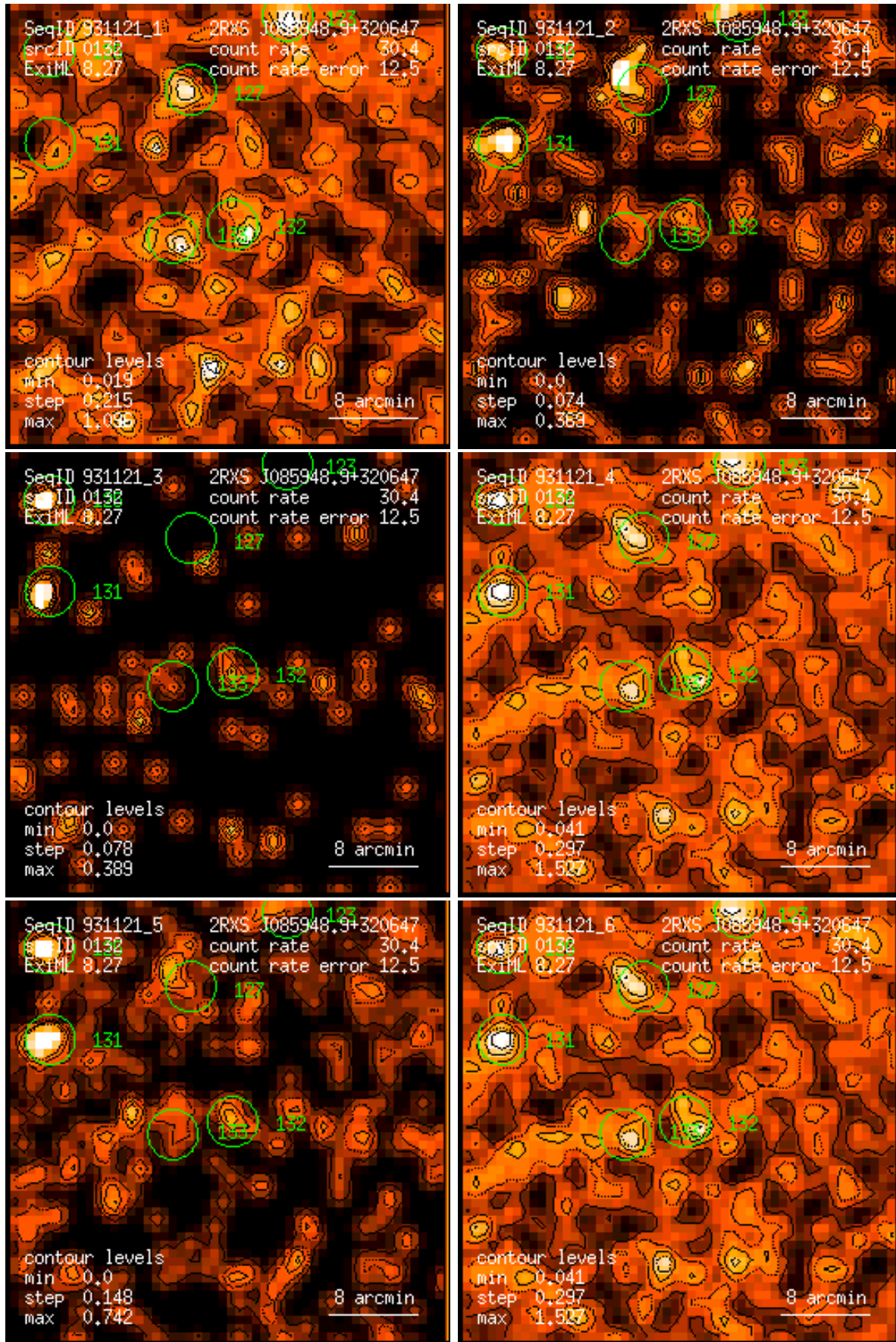
Figure 132: RASS 931121: detection 0132: band rate images, Gaussian filter: (1) PSPC channels 11 – 41, (2) 52 – 90, (3) 91 – 201, (4) 11 – 235, (5) 52 – 201, (6) 11 – 201. Broad band rates in counts/ks. Band rate contour levels in counts/ks/arcmin 2 .
