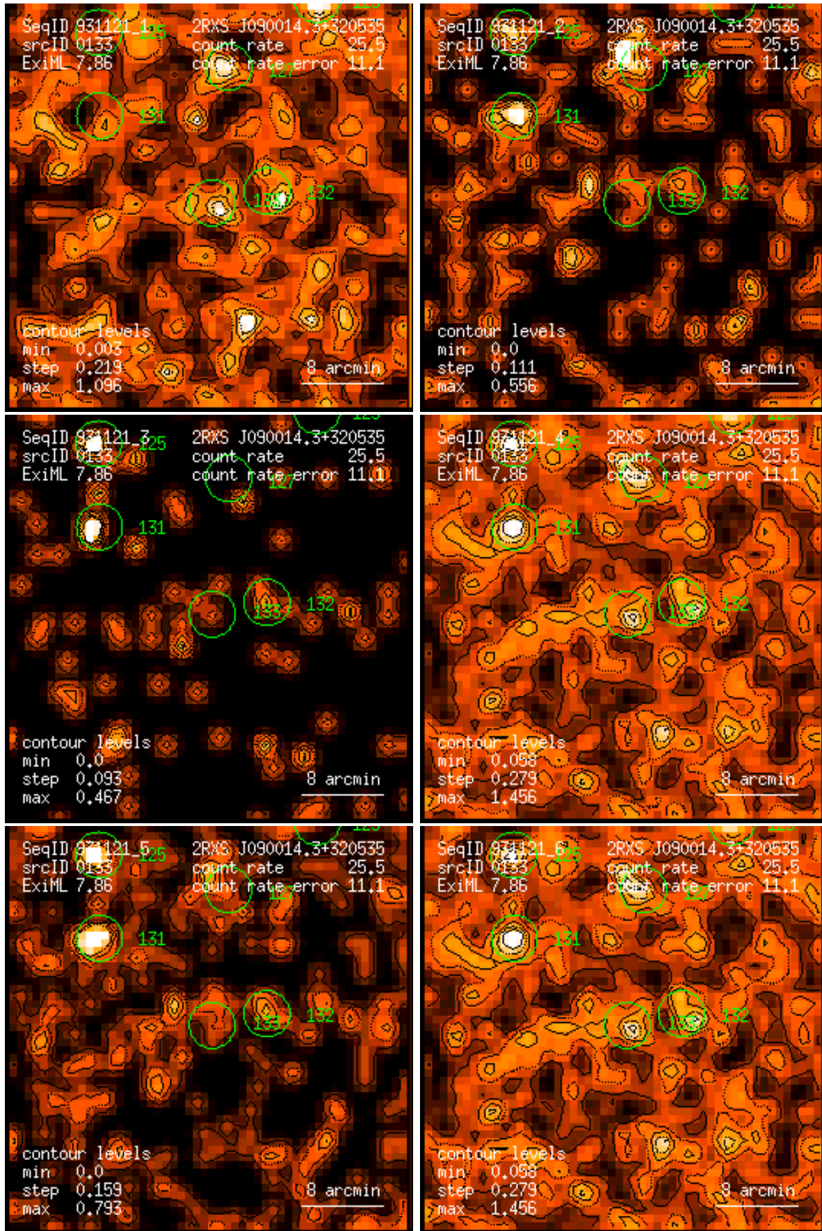
Figure 133: RASS 931121: detection 0133: band rate images, Gaussian filter: (1) PSPC channels 11 – 41, (2) 52 – 90, (3) 91 – 201, (4) 11 – 235, (5) 52 – 201, (6) 11 – 201. Broad band rates in counts/ks. Band rate contour levels in counts/ks/arcmin 2 .
