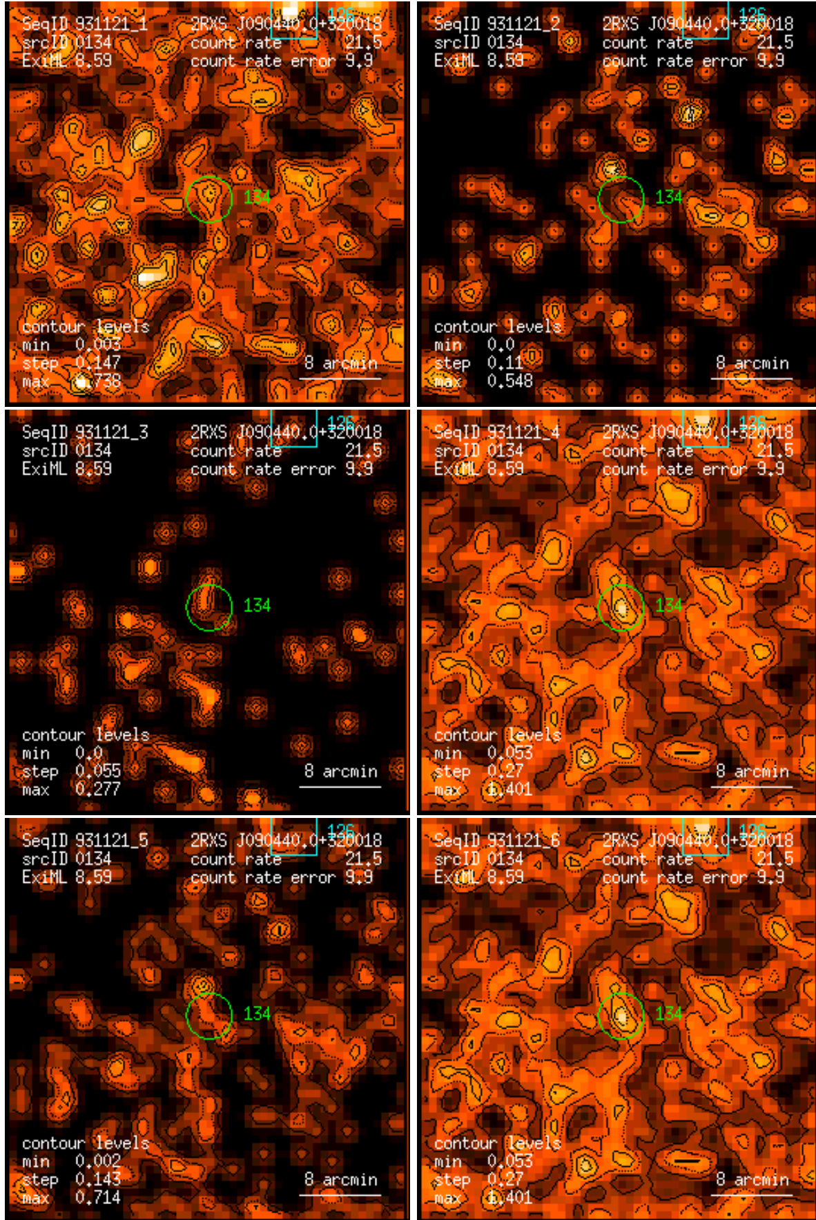
Figure 134: RASS 931121: detection 0134: band rate images, Gaussian filter: (1) PSPC channels 11 – 41, (2) 52 – 90, (3) 91 – 201, (4) 11 – 235, (5) 52 – 201, (6) 11 – 201. Broad band rates in counts/ks. Band rate contour levels in counts/ks/arcmin 2 .
