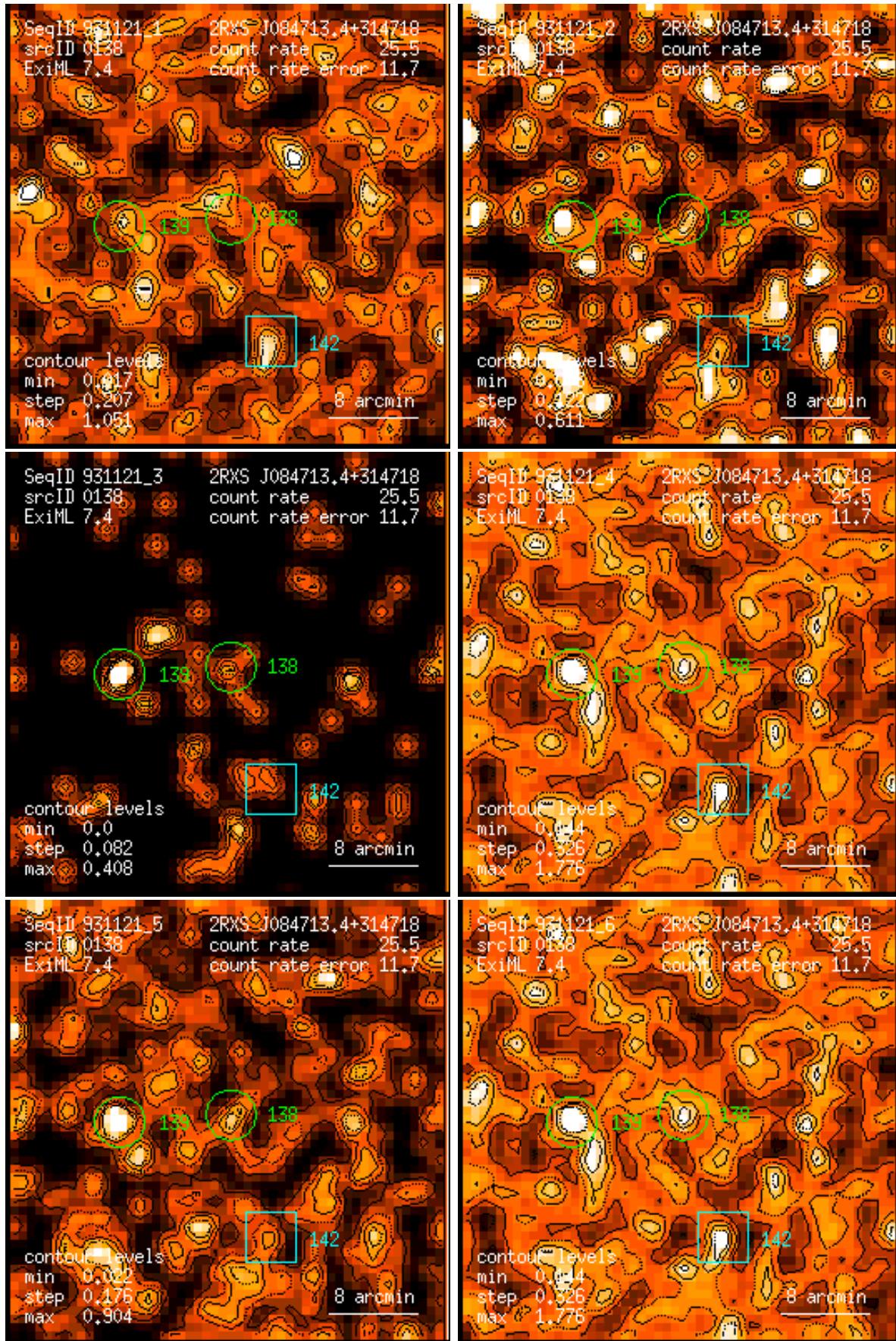
Figure 138: RASS 931121: detection 0138: band rate images, Gaussian filter: (1) PSPC channels 11 – 41, (2) 52 – 90, (3) 91 – 201, (4) 11 – 235, (5) 52 – 201, (6) 11 – 201. Broad band rates in counts/ks. Band rate contour levels in counts/ks/arcmin 2 .
