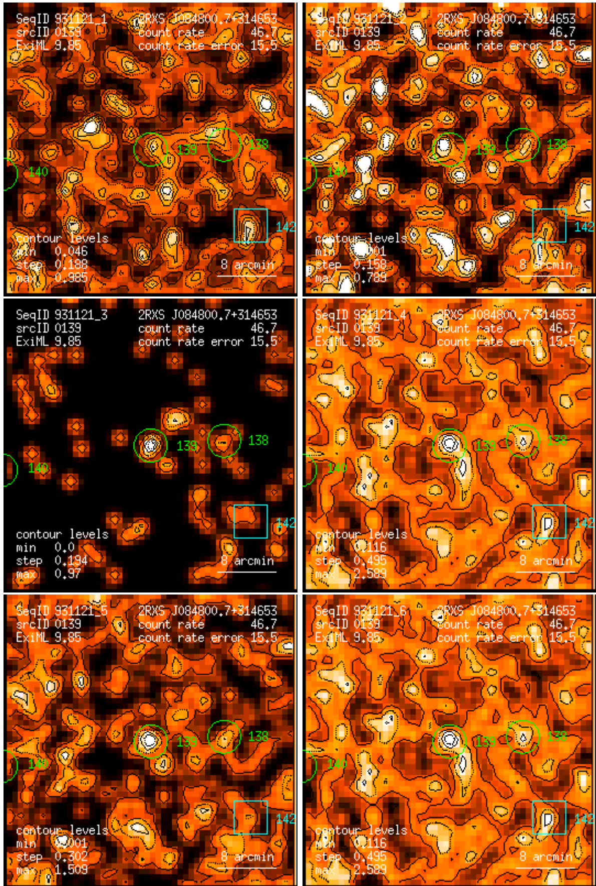
Figure 139: RASS 931121: detection 0139: band rate images, Gaussian filter: (1) PSPC channels 11 – 41, (2) 52 – 90, (3) 91 – 201, (4) 11 – 235, (5) 52 – 201, (6) 11 – 201. Broad band rates in counts/ks. Band rate contour levels in counts/ks/arcmin 2 .
