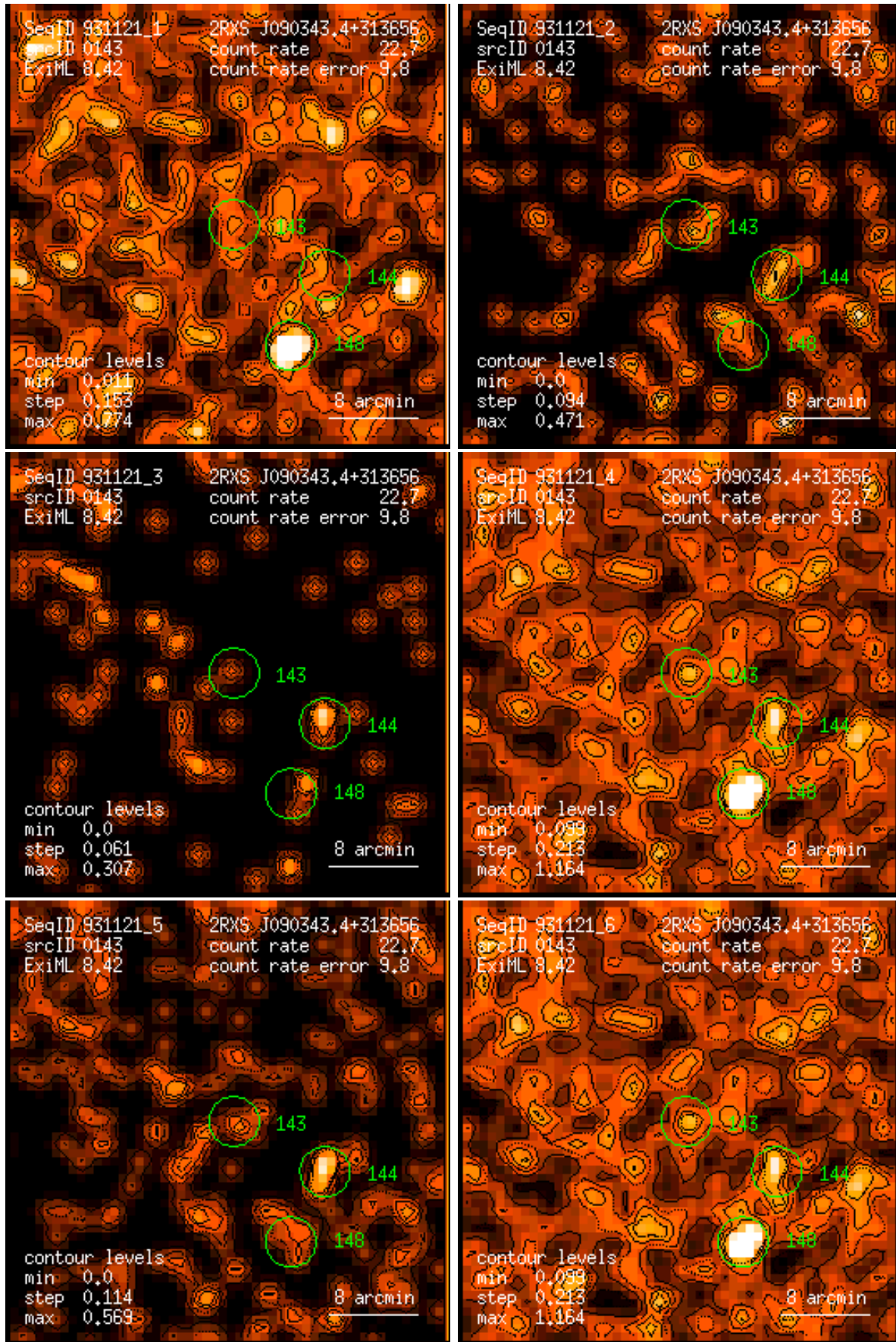
Figure 143: RASS 931121: detection 0143: band rate images, Gaussian filter: (1) PSPC channels 11 – 41, (2) 52 – 90, (3) 91 – 201, (4) 11 – 235, (5) 52 – 201, (6) 11 – 201. Broad band rates in counts/ks. Band rate contour levels in counts/ks/arcmin 2 .
