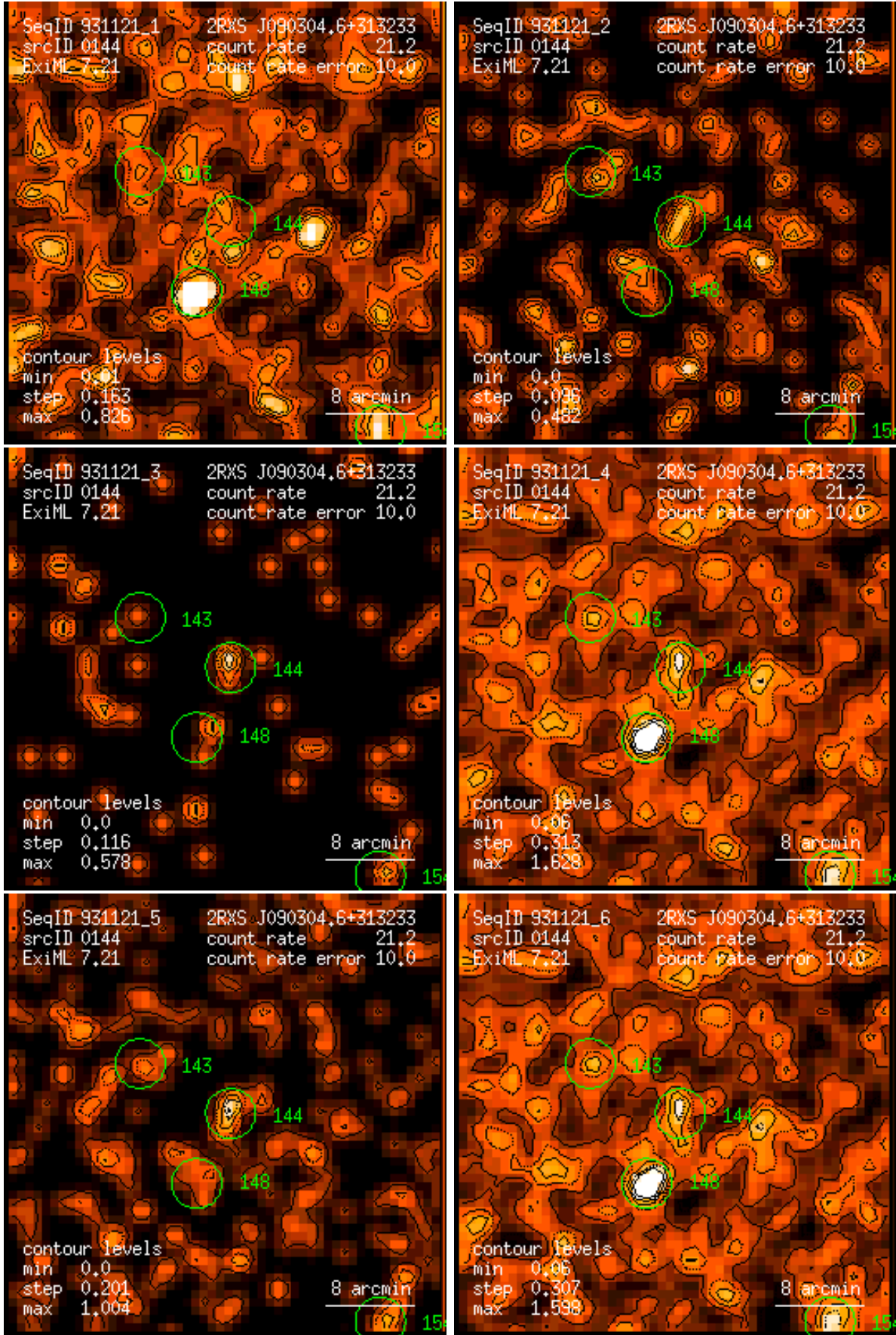
Figure 144: RASS 931121: detection 0144: band rate images, Gaussian filter: (1) PSPC channels 11 – 41, (2) 52 – 90, (3) 91 – 201, (4) 11 – 235, (5) 52 – 201, (6) 11 – 201. Broad band rates in counts/ks. Band rate contour levels in counts/ks/arcmin 2 .
