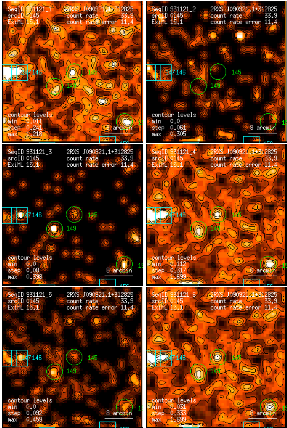
Figure 145: RASS 931121: detection 0145: band rate images, Gaussian filter: (1) PSPC channels 11 – 41, (2) 52 – 90, (3) 91 – 201, (4) 11 – 235, (5) 52 – 201, (6) 11 – 201. Broad band rates in counts/ks. Band rate contour levels in counts/ks/arcmin 2 .
