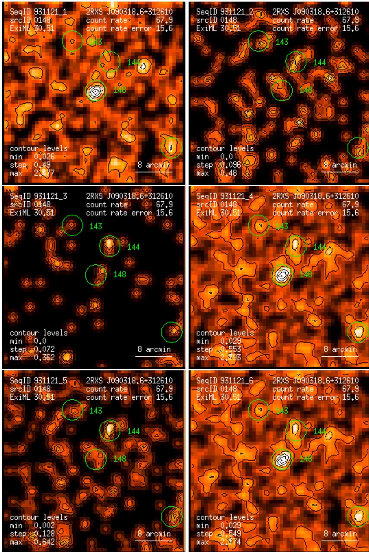
Figure 148: RASS 931121: detection 0148: band rate images, Gaussian filter: (1) PSPC channels 11 – 41, (2) 52 – 90, (3) 91 – 201, (4) 11 – 235, (5) 52 – 201, (6) 11 – 201. Broad band rates in counts/ks. Band rate contour levels in counts/ks/arcmin 2 .
