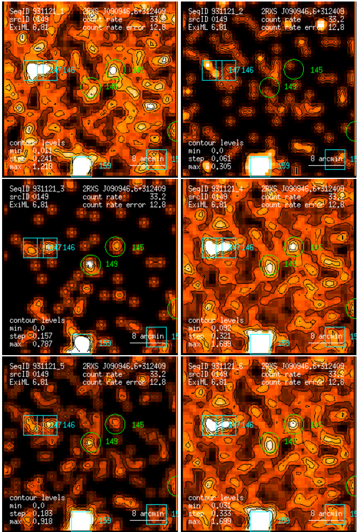
Figure 149: RASS 931121: detection 0149: band rate images, Gaussian filter: (1) PSPC channels 11 – 41, (2) 52 – 90, (3) 91 – 201, (4) 11 – 235, (5) 52 – 201, (6) 11 – 201. Broad band rates in counts/ks. Band rate contour levels in counts/ks/arcmin 2 .
