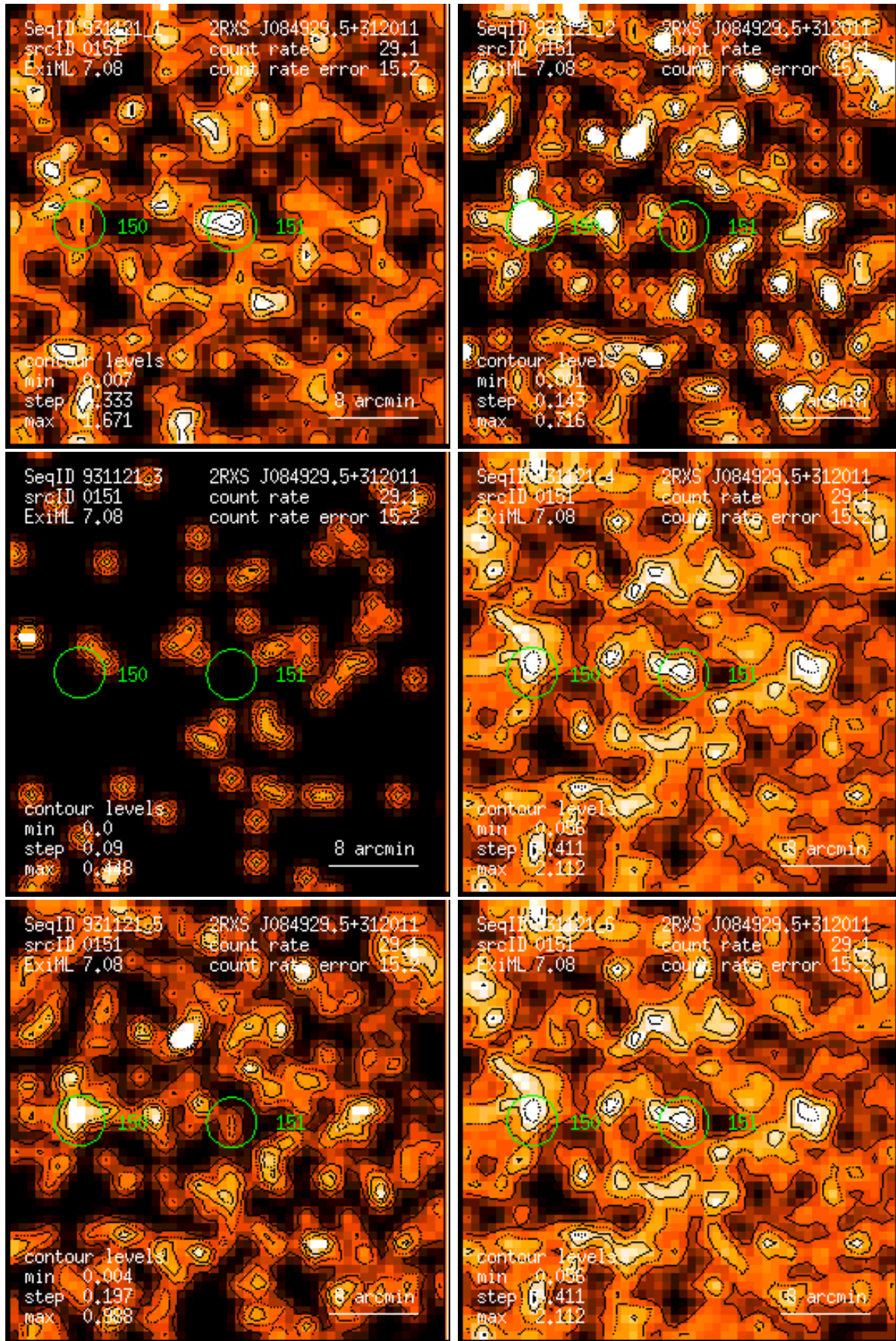
Figure 151: RASS 931121: detection 0151: band rate images, Gaussian filter: (1) PSPC channels 11 – 41, (2) 52 – 90, (3) 91 – 201, (4) 11 – 235, (5) 52 – 201, (6) 11 – 201. Broad band rates in counts/ks. Band rate contour levels in counts/ks/arcmin 2 .
