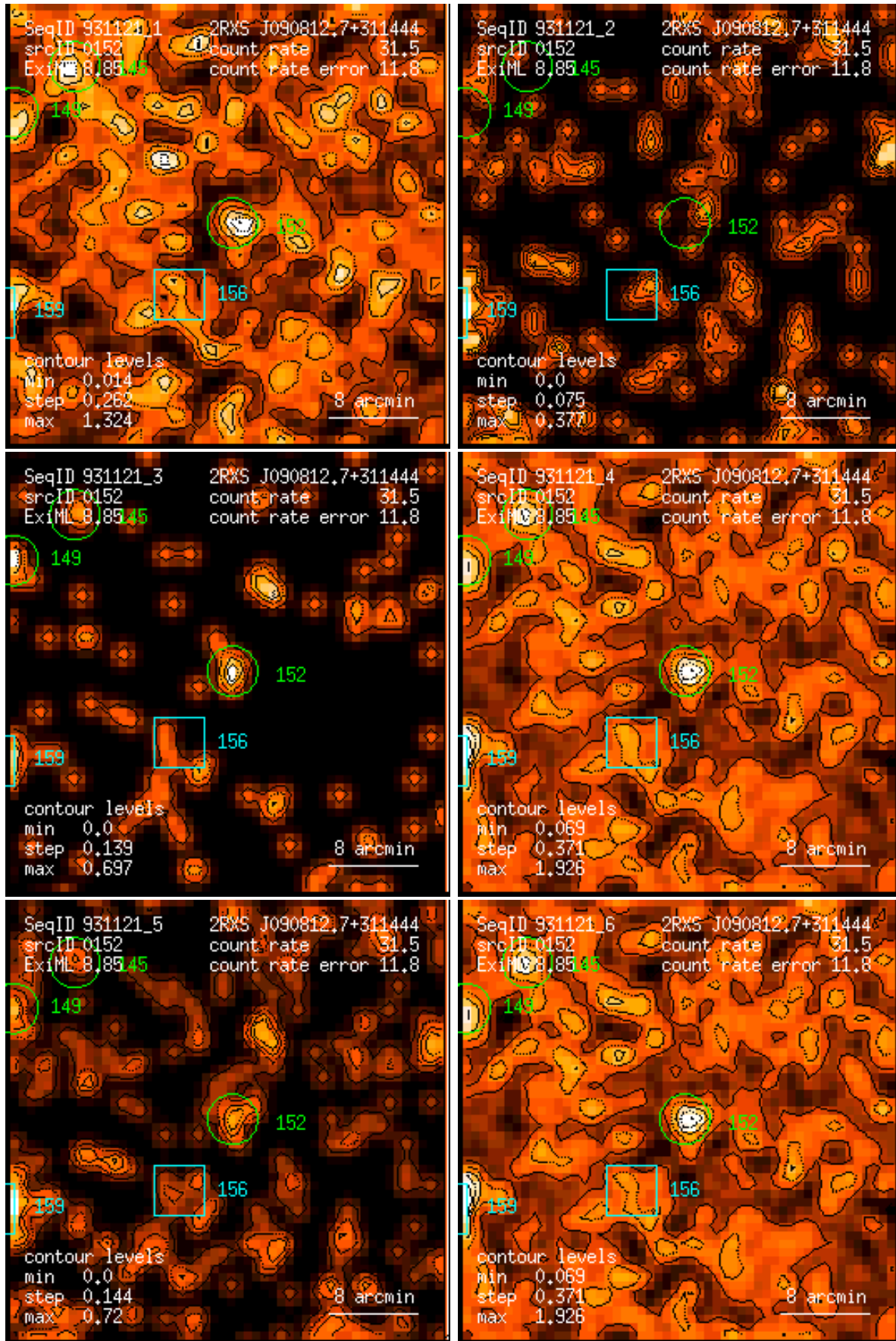
Figure 152: RASS 931121: detection 0152: band rate images, Gaussian filter: (1) PSPC channels 11 – 41, (2) 52 – 90, (3) 91 – 201, (4) 11 – 235, (5) 52 – 201, (6) 11 – 201. Broad band rates in counts/ks. Band rate contour levels in counts/ks/arcmin 2 .
