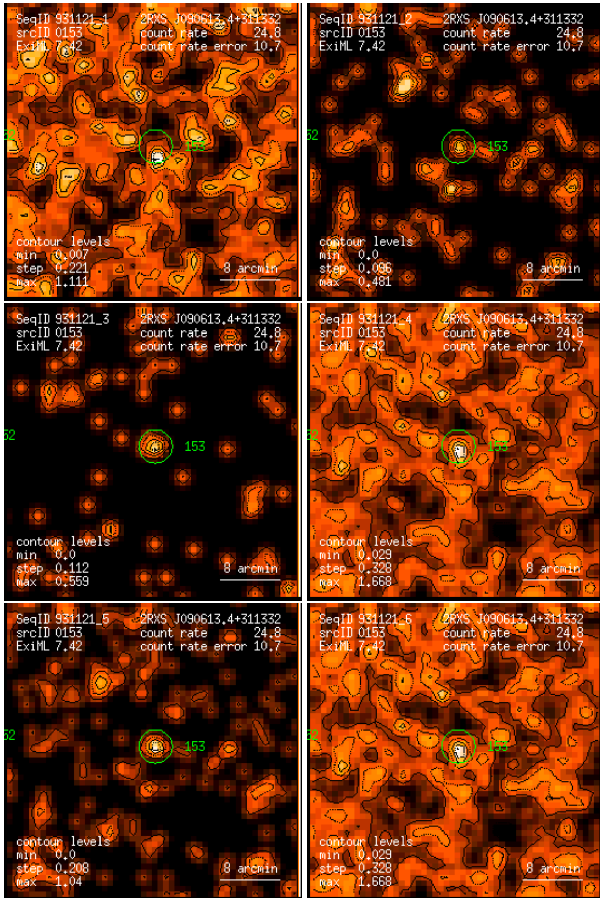
Figure 153: RASS 931121: detection 0153: band rate images, Gaussian filter: (1) PSPC channels 11 – 41, (2) 52 – 90, (3) 91 – 201, (4) 11 – 235, (5) 52 – 201, (6) 11 – 201. Broad band rates in counts/ks. Band rate contour levels in counts/ks/arcmin 2 .
