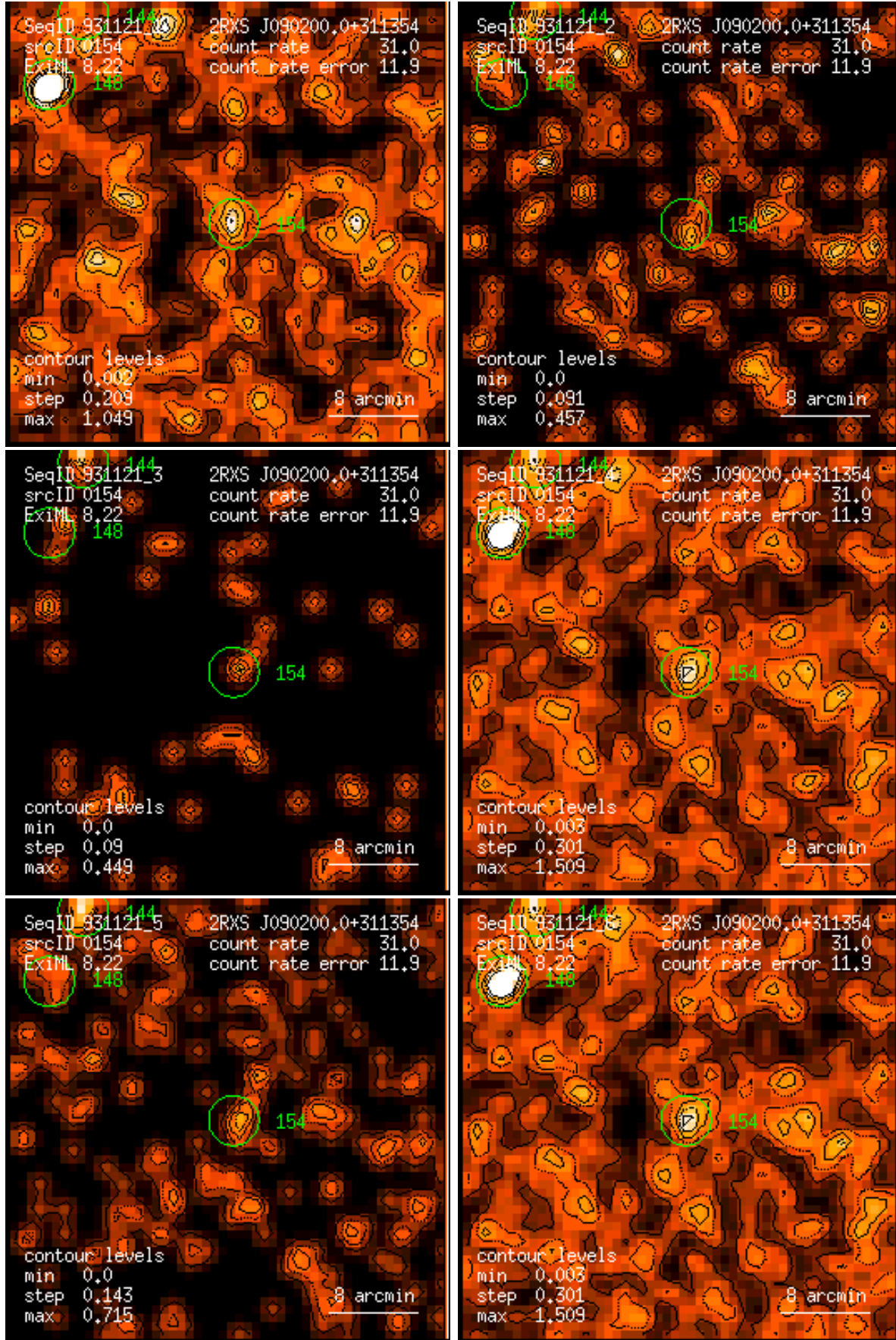
Figure 154: RASS 931121: detection 0154: band rate images, Gaussian filter: (1) PSPC channels 11 – 41, (2) 52 – 90, (3) 91 – 201, (4) 11 – 235, (5) 52 – 201, (6) 11 – 201. Broad band rates in counts/ks. Band rate contour levels in counts/ks/arcmin 2 .
