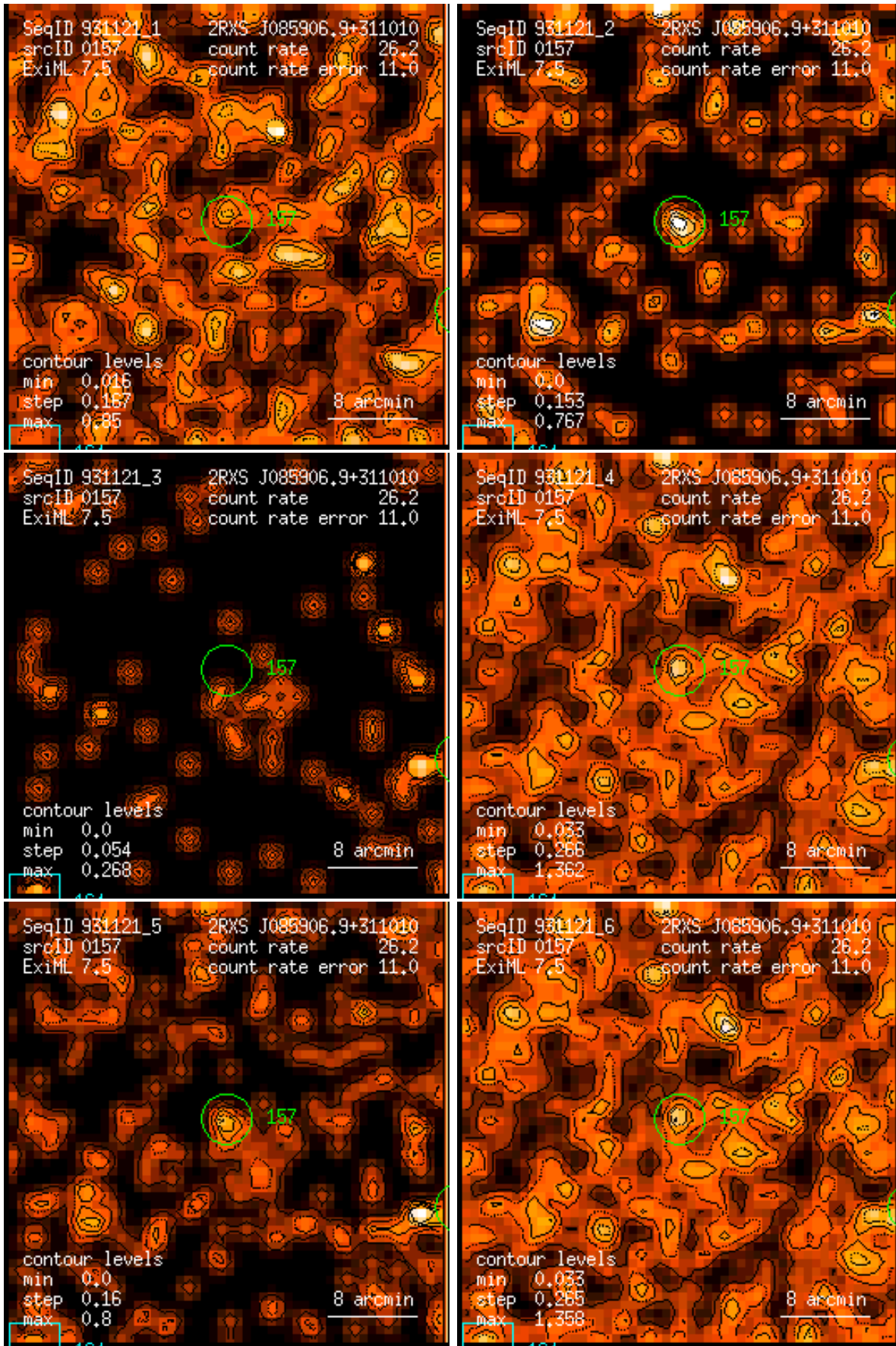
Figure 157: RASS 931121: detection 0157: band rate images, Gaussian filter: (1) PSPC channels 11 – 41, (2) 52 – 90, (3) 91 – 201, (4) 11 – 235, (5) 52 – 201, (6) 11 – 201. Broad band rates in counts/ks. Band rate contour levels in counts/ks/arcmin 2 .
