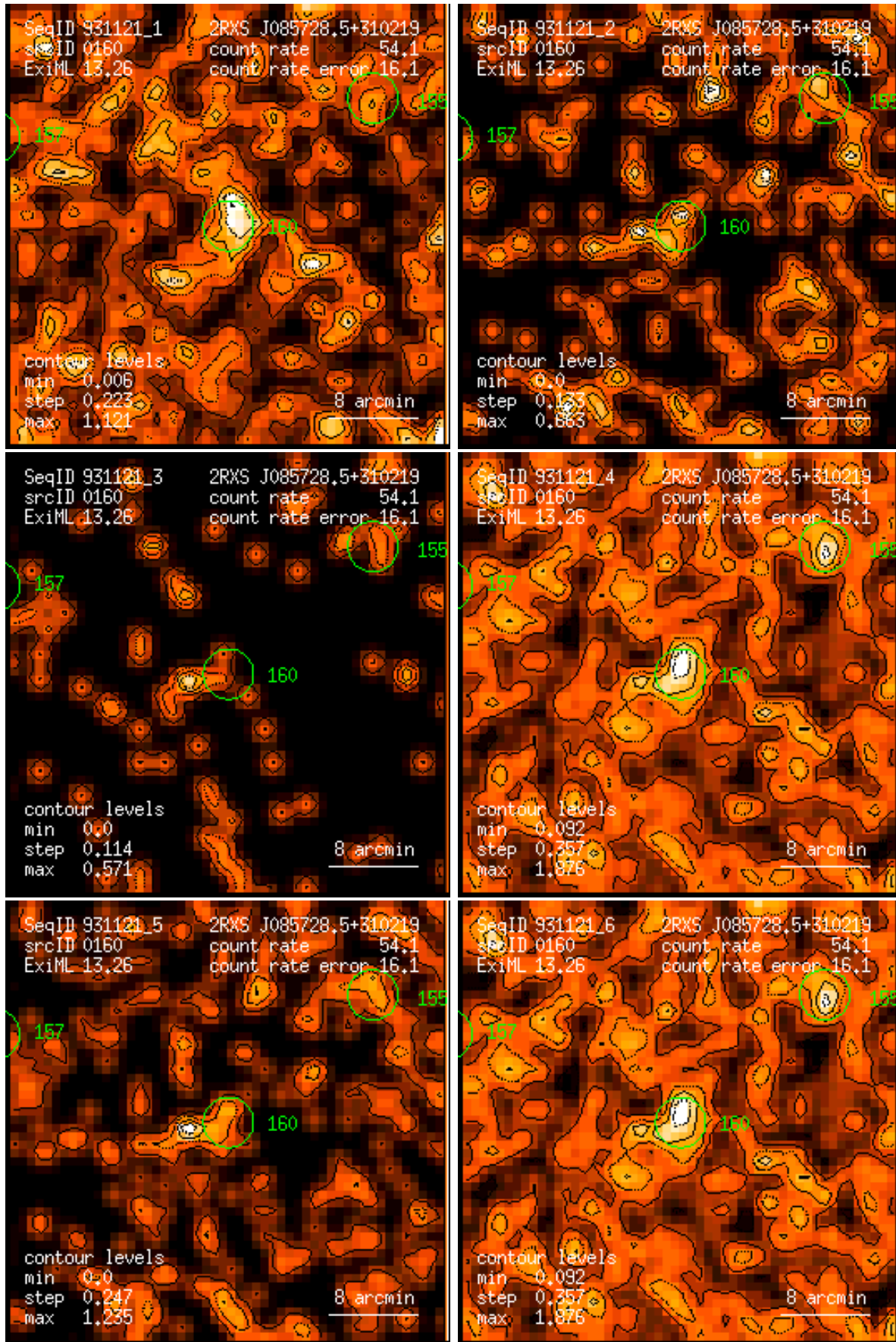
Figure 160: RASS 931121: detection 0160: band rate images, Gaussian filter: (1) PSPC channels 11 – 41, (2) 52 – 90, (3) 91 – 201, (4) 11 – 235, (5) 52 – 201, (6) 11 – 201. Broad band rates in counts/ks. Band rate contour levels in counts/ks/arcmin 2 .
