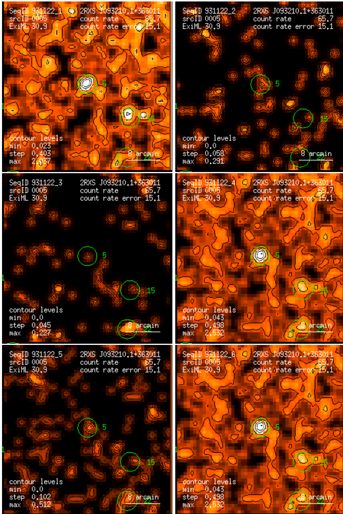
Figure 5: RASS 931122: detection 0005: band rate images, Gaussian filter: (1) PSPC channels 11 – 41, (2) 52 – 90, (3) 91 – 201, (4) 11 – 235, (5) 52 – 201, (6) 11 – 201. Broad band rates in counts/ks. Band rate contour levels in counts/ks/arcmin 2 .
