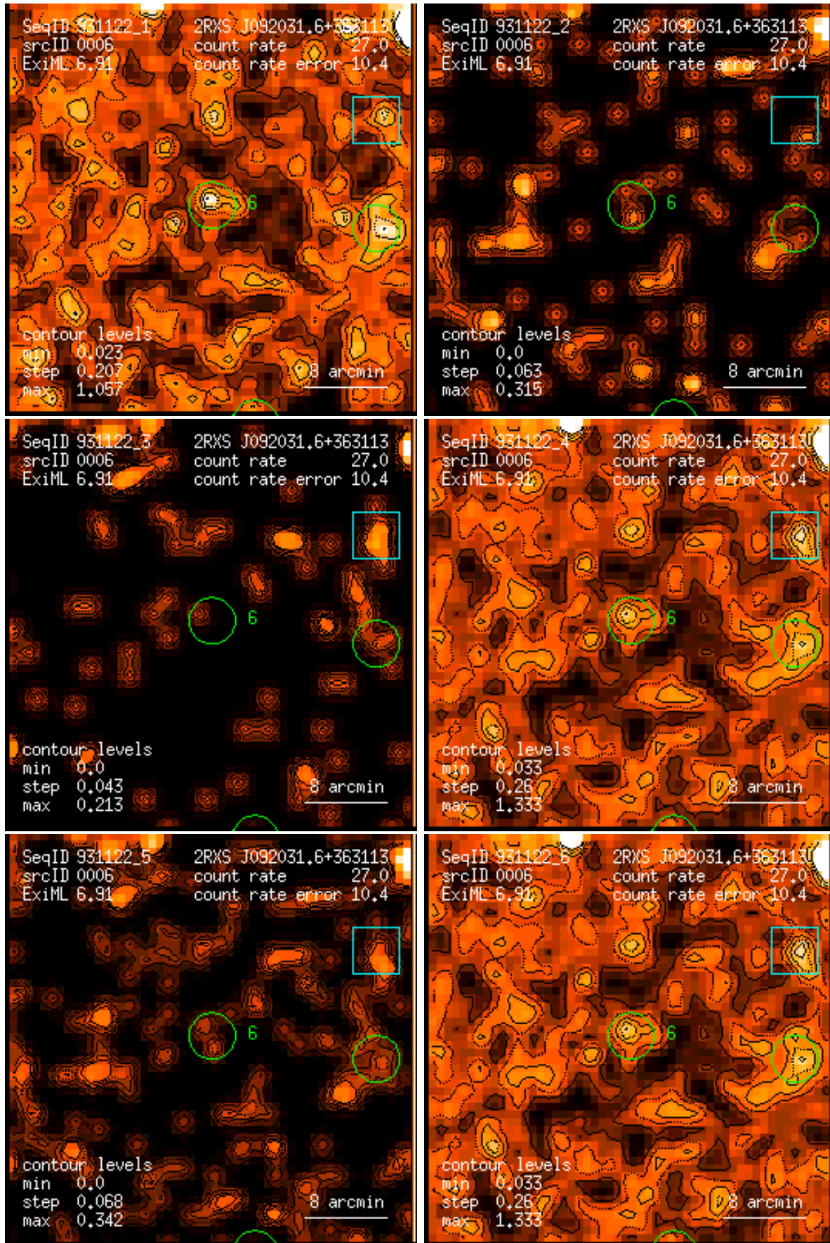
Figure 6: RASS 931122: detection 0006: band rate images, Gaussian filter: (1) PSPC channels 11 – 41, (2) 52 – 90, (3) 91 – 201, (4) 11 – 235, (5) 52 – 201, (6) 11 – 201. Broad band rates in counts/ks. Band rate contour levels in counts/ks/arcmin 2 .
