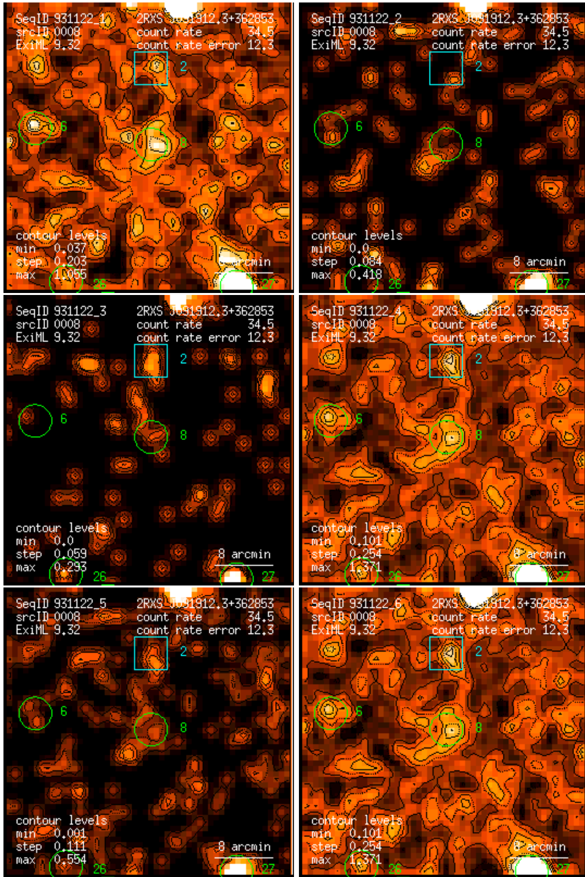
Figure 8: RASS 931122: detection 0008: band rate images, Gaussian filter: (1) PSPC channels 11 – 41, (2) 52 – 90, (3) 91 – 201, (4) 11 – 235, (5) 52 – 201, (6) 11 – 201. Broad band rates in counts/ks. Band rate contour levels in counts/ks/arcmin 2 .
