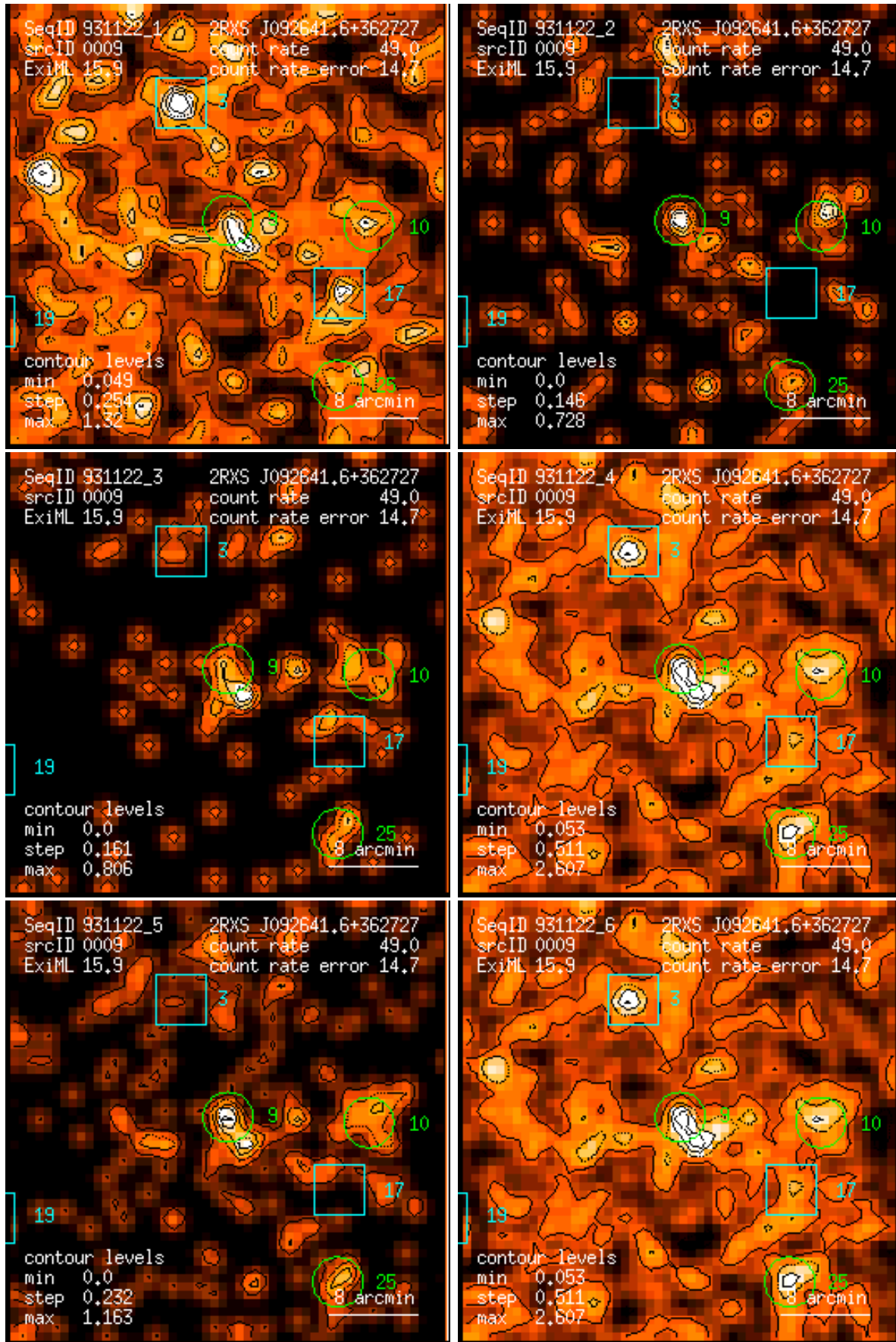
Figure 9: RASS 931122: detection 0009: band rate images, Gaussian filter: (1) PSPC channels 11 – 41, (2) 52 – 90, (3) 91 – 201, (4) 11 – 235, (5) 52 – 201, (6) 11 – 201. Broad band rates in counts/ks. Band rate contour levels in counts/ks/arcmin 2 .
