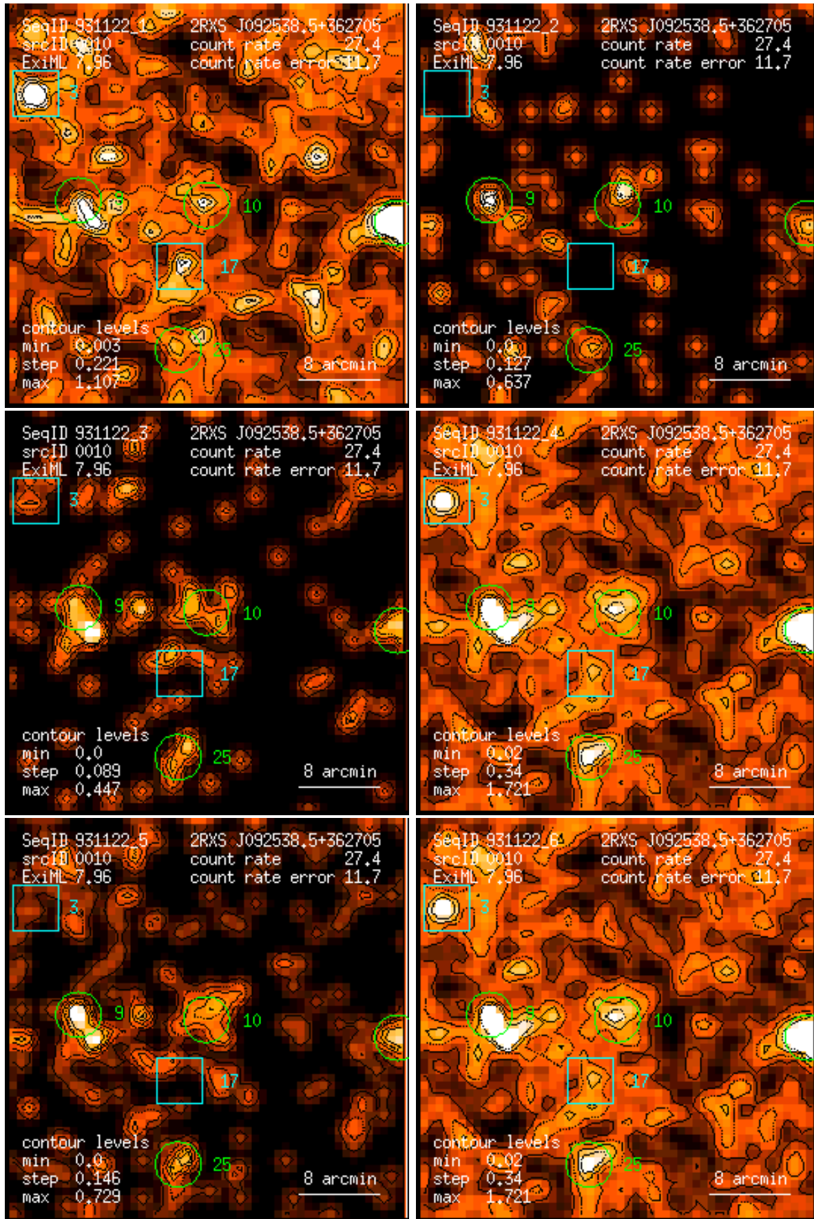
Figure 10: RASS 931122: detection 0010: band rate images, Gaussian filter: (1) PSPC channels 11 – 41, (2) 52 – 90, (3) 91 – 201, (4) 11 – 235, (5) 52 – 201, (6) 11 – 201. Broad band rates in counts/ks. Band rate contour levels in counts/ks/arcmin 2 .
