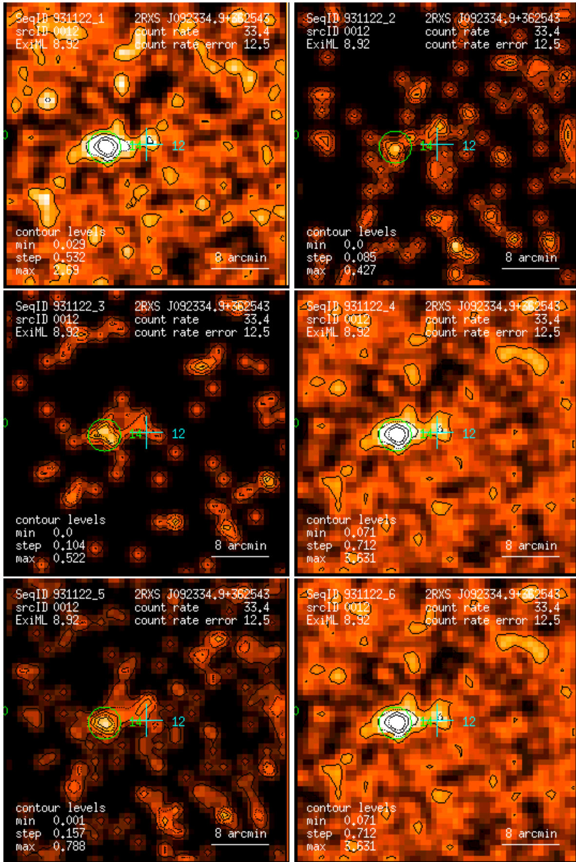
Figure 12: RASS 931122: detection 0012: band rate images, Gaussian filter: (1) PSPC channels 11 – 41, (2) 52 – 90, (3) 91 – 201, (4) 11 – 235, (5) 52 – 201, (6) 11 – 201. Broad band rates in counts/ks. Band rate contour levels in counts/ks/arcmin 2 .
