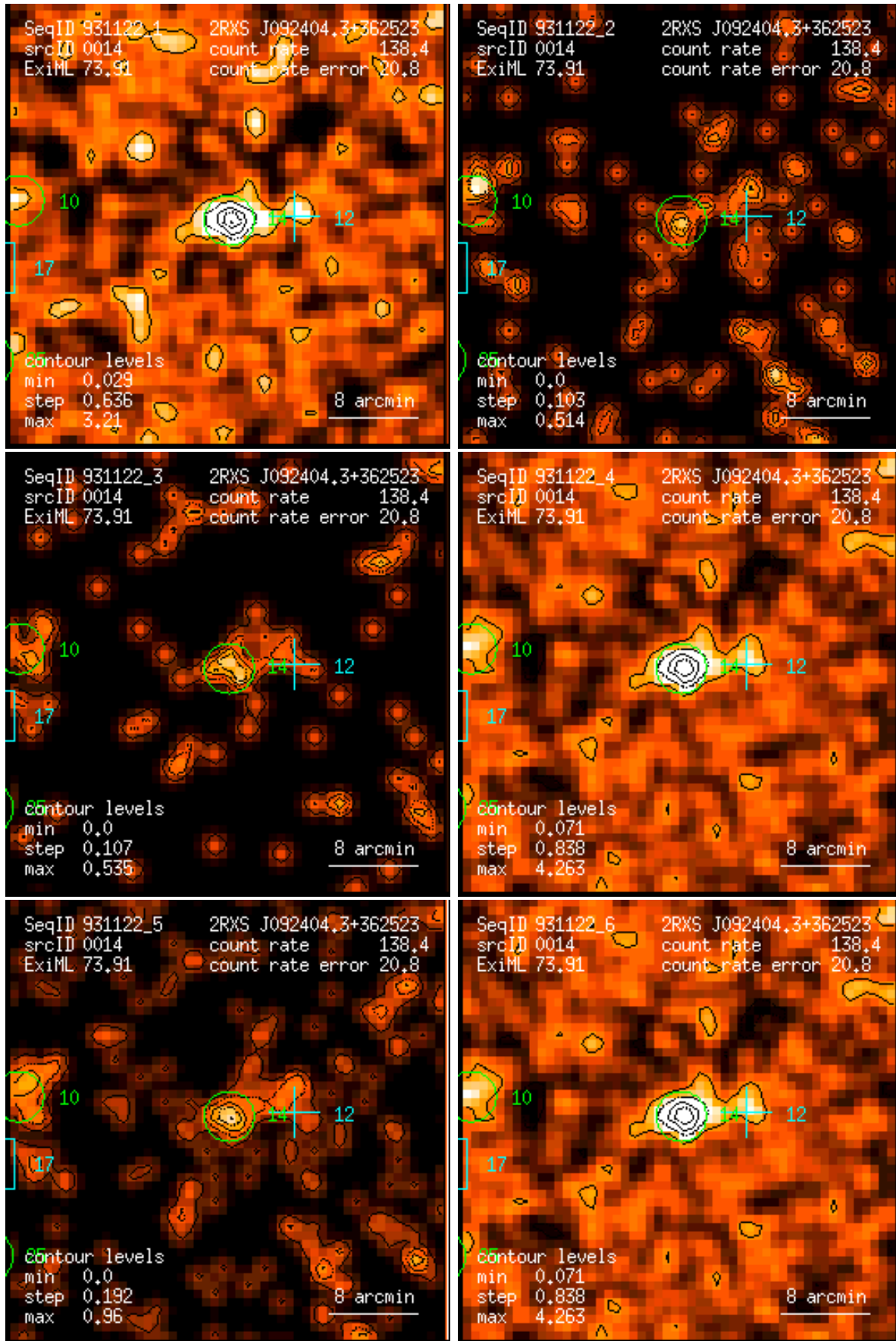
Figure 14: RASS 931122: detection 0014: band rate images, Gaussian filter: (1) PSPC channels 11 – 41, (2) 52 – 90, (3) 91 – 201, (4) 11 – 235, (5) 52 – 201, (6) 11 – 201. Broad band rates in counts/ks. Band rate contour levels in counts/ks/arcmin 2 .
