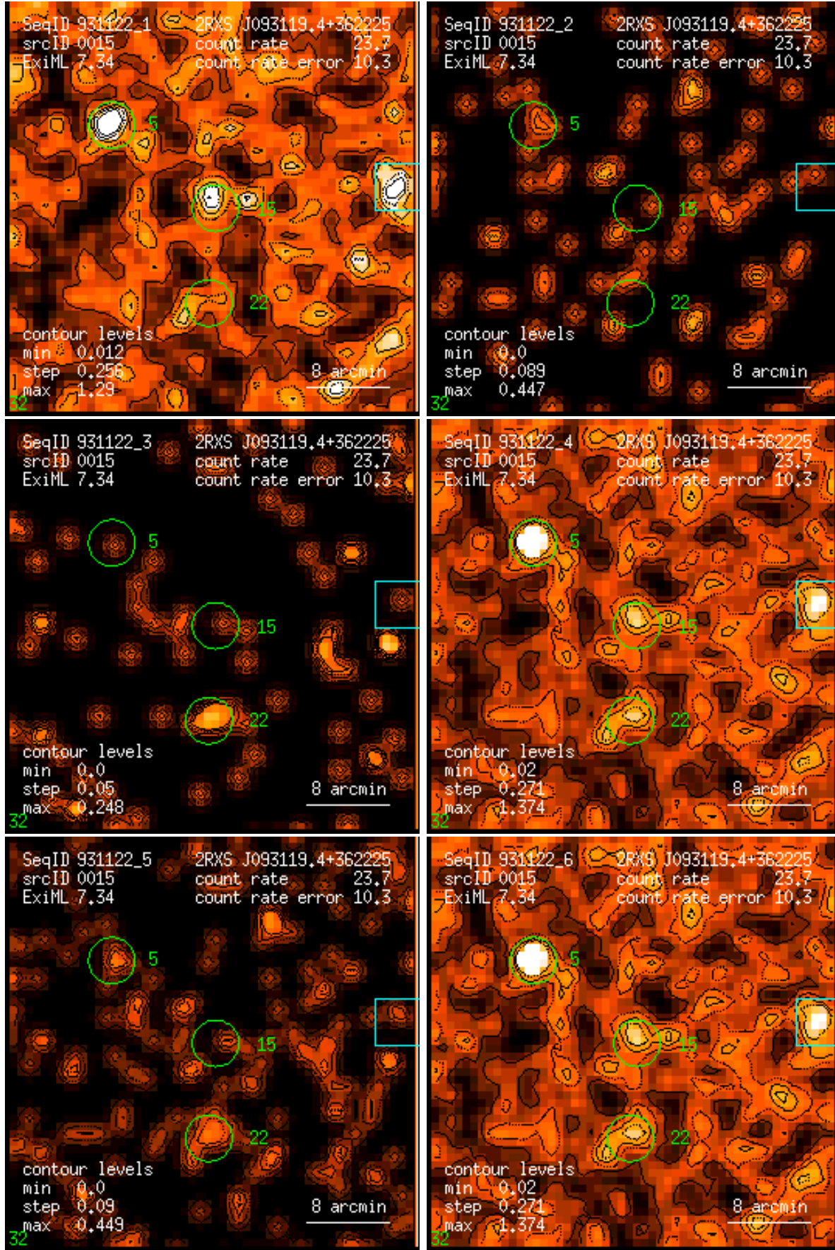
Figure 15: RASS 931122: detection 0015: band rate images, Gaussian filter: (1) PSPC channels 11 – 41, (2) 52 – 90, (3) 91 – 201, (4) 11 – 235, (5) 52 – 201, (6) 11 – 201. Broad band rates in counts/ks. Band rate contour levels in counts/ks/arcmin 2 .
