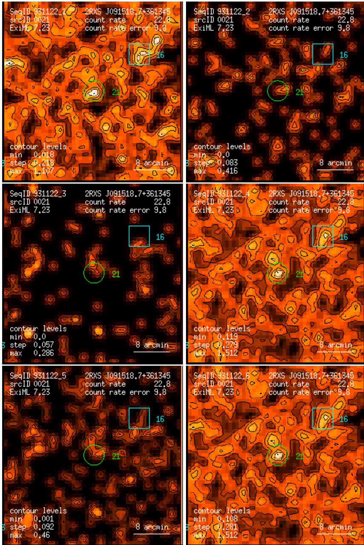
Figure 21: RASS 931122: detection 0021: band rate images, Gaussian filter: (1) PSPC channels 11 – 41, (2) 52 – 90, (3) 91 – 201, (4) 11 – 235, (5) 52 – 201, (6) 11 – 201. Broad band rates in counts/ks. Band rate contour levels in counts/ks/arcmin 2 .
