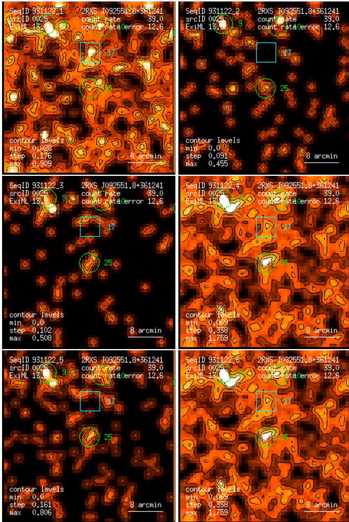
Figure 25: RASS 931122: detection 0025: band rate images, Gaussian filter: (1) PSPC channels 11 – 41, (2) 52 – 90, (3) 91 – 201, (4) 11 – 235, (5) 52 – 201, (6) 11 – 201. Broad band rates in counts/ks. Band rate contour levels in counts/ks/arcmin 2 .
