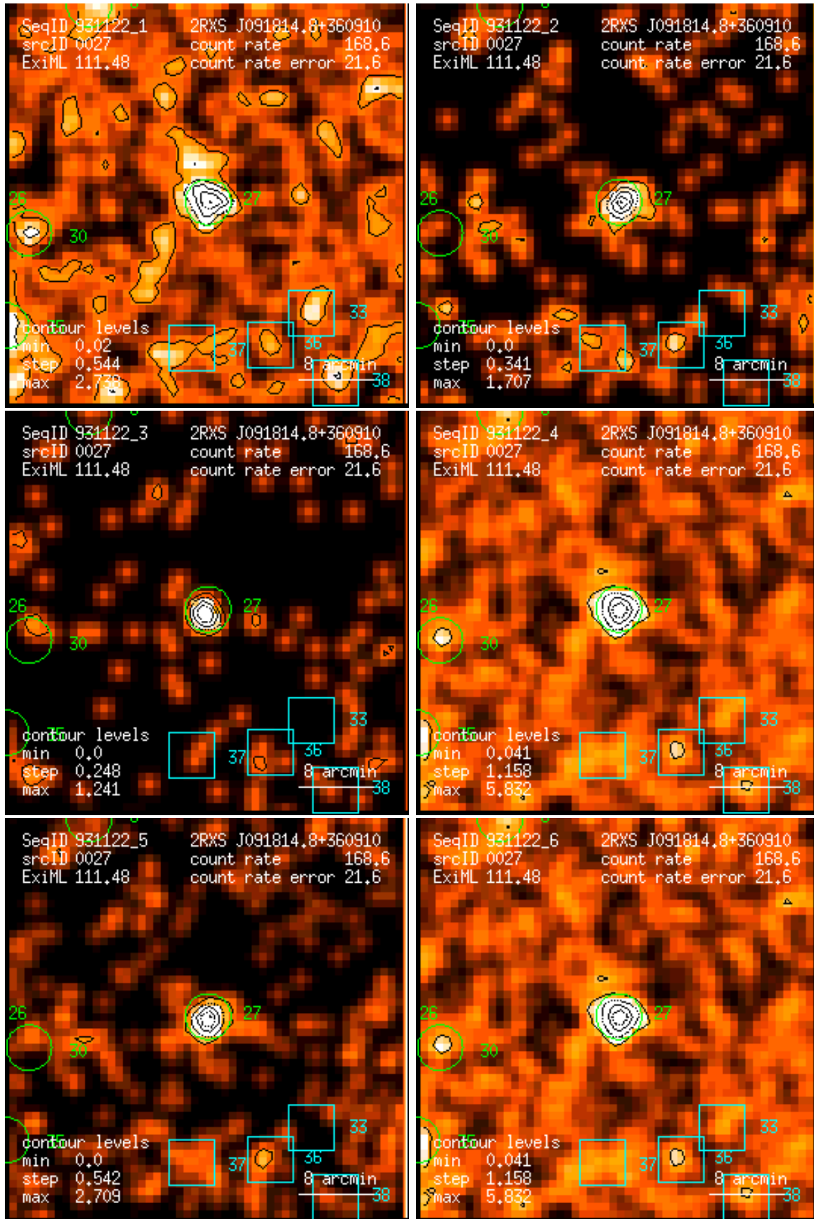
Figure 27: RASS 931122: detection 0027: band rate images, Gaussian filter: (1) PSPC channels 11 – 41, (2) 52 – 90, (3) 91 – 201, (4) 11 – 235, (5) 52 – 201, (6) 11 – 201. Broad band rates in counts/ks. Band rate contour levels in counts/ks/arcmin 2 .
