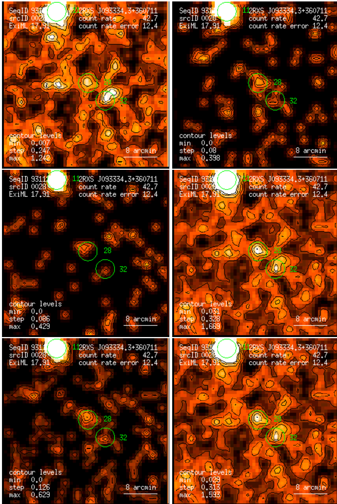
Figure 28: RASS 931122: detection 0028: band rate images, Gaussian filter: (1) PSPC channels 11 – 41, (2) 52 – 90, (3) 91 – 201, (4) 11 – 235, (5) 52 – 201, (6) 11 – 201. Broad band rates in counts/ks. Band rate contour levels in counts/ks/arcmin 2 .
