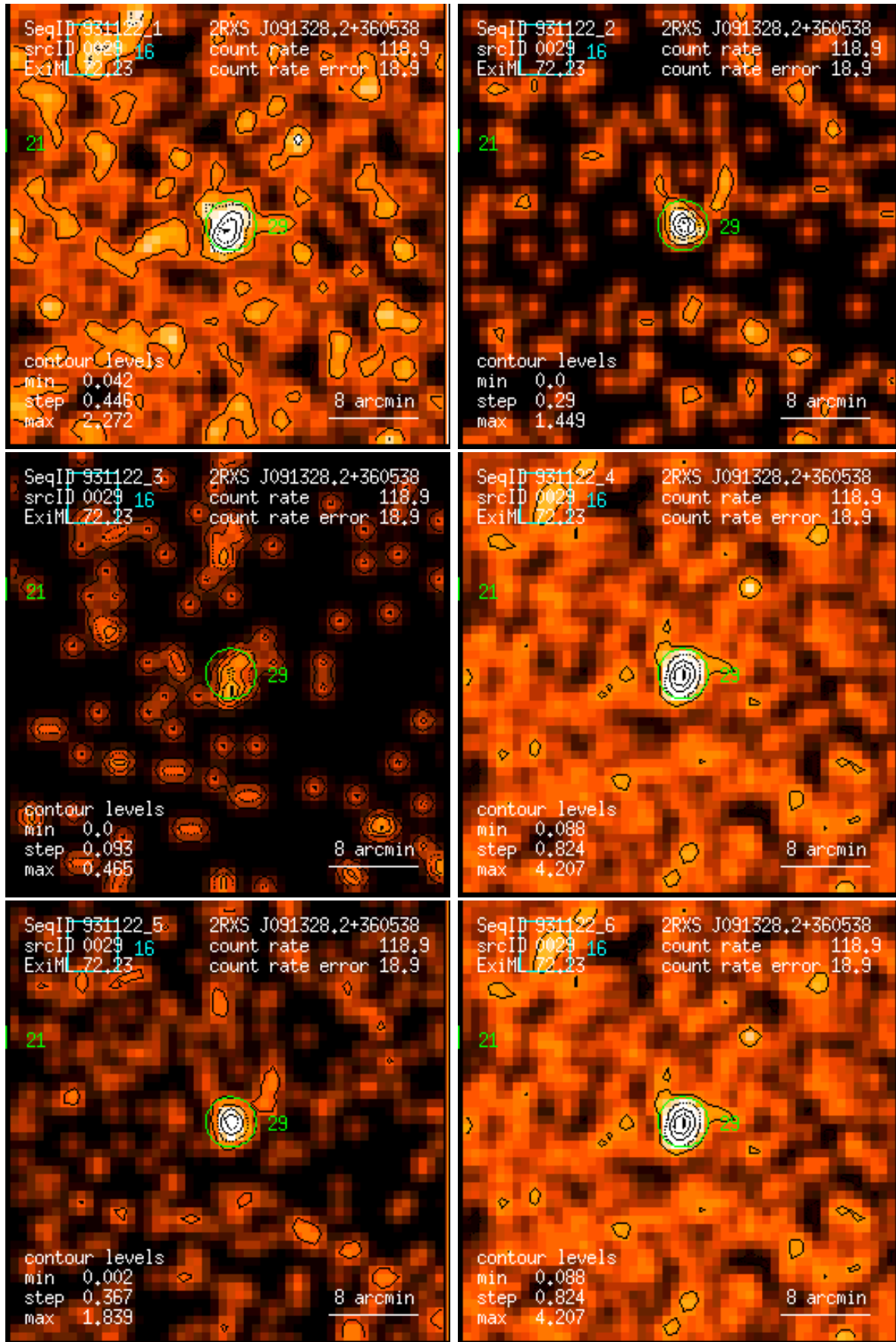
Figure 29: RASS 931122: detection 0029: band rate images, Gaussian filter: (1) PSPC channels 11 – 41, (2) 52 – 90, (3) 91 – 201, (4) 11 – 235, (5) 52 – 201, (6) 11 – 201. Broad band rates in counts/ks. Band rate contour levels in counts/ks/arcmin 2 .
