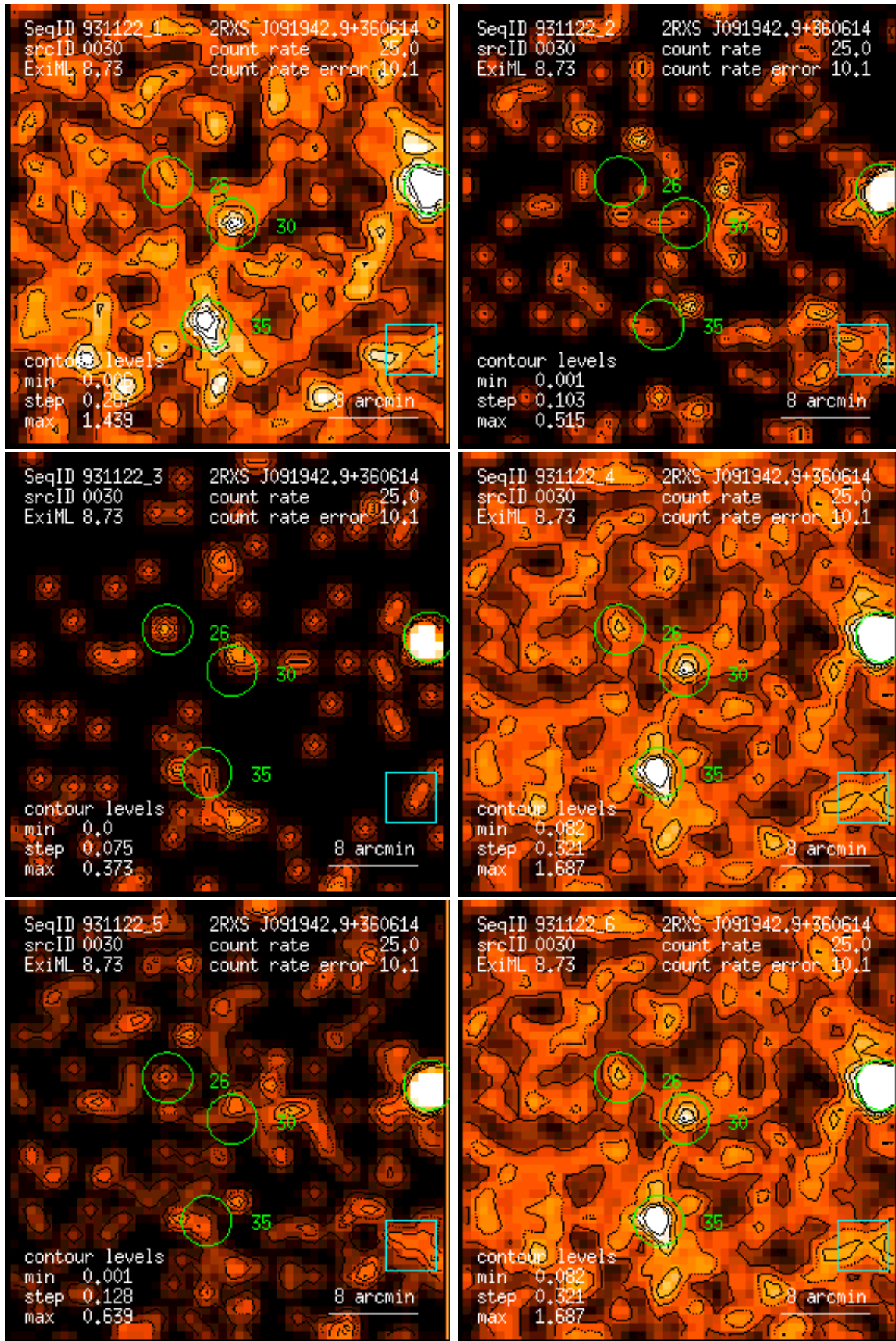
Figure 30: RASS 931122: detection 0030: band rate images, Gaussian filter: (1) PSPC channels 11 – 41, (2) 52 – 90, (3) 91 – 201, (4) 11 – 235, (5) 52 – 201, (6) 11 – 201. Broad band rates in counts/ks. Band rate contour levels in counts/ks/arcmin 2 .
