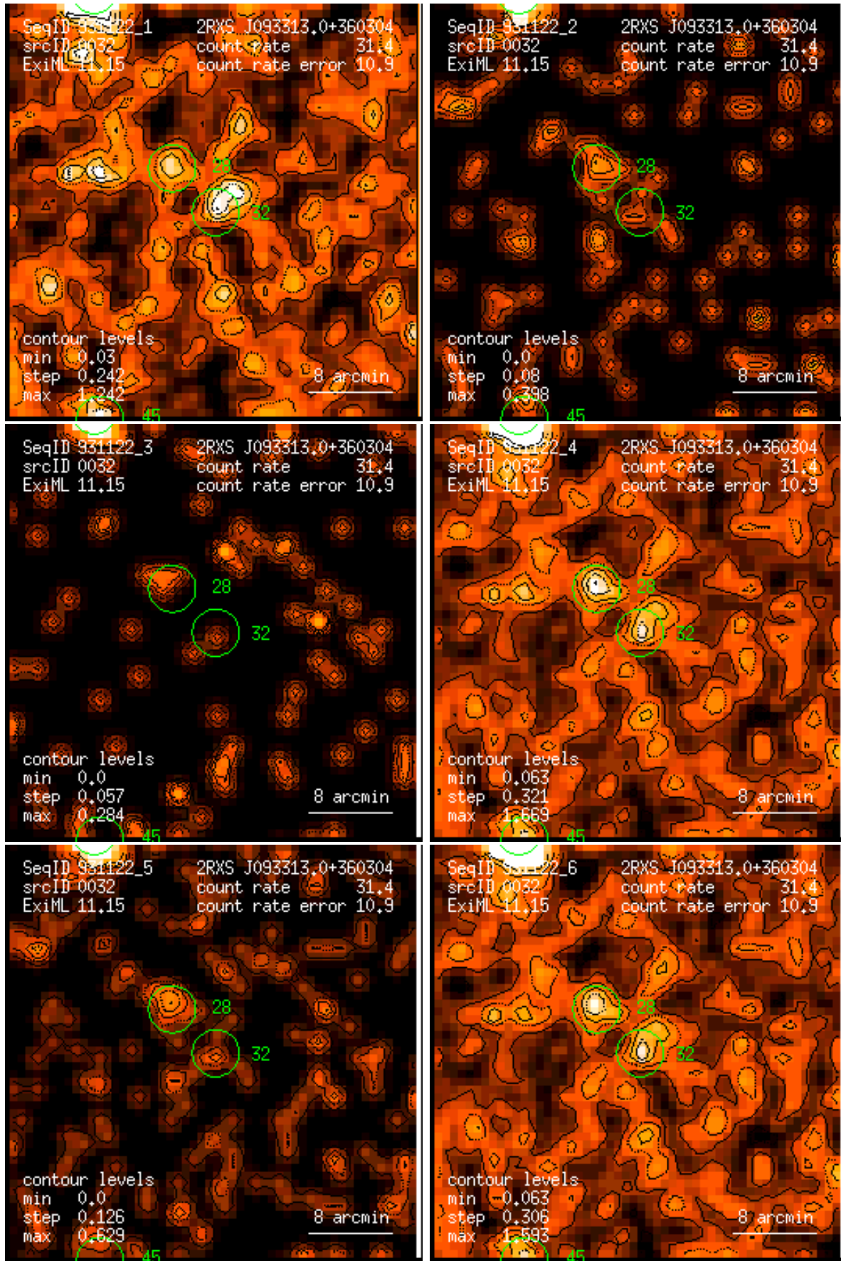
Figure 32: RASS 931122: detection 0032: band rate images, Gaussian filter: (1) PSPC channels 11 – 41, (2) 52 – 90, (3) 91 – 201, (4) 11 – 235, (5) 52 – 201, (6) 11 – 201. Broad band rates in counts/ks. Band rate contour levels in counts/ks/arcmin 2 .
