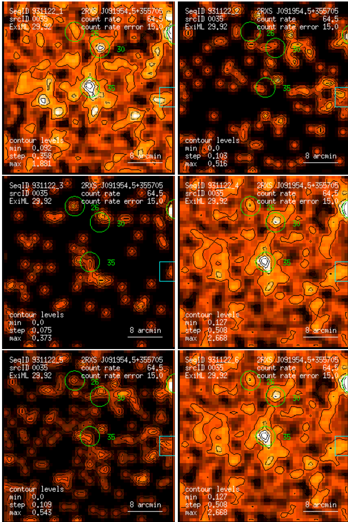
Figure 35: RASS 931122: detection 0035: band rate images, Gaussian filter: (1) PSPC channels 11 – 41, (2) 52 – 90, (3) 91 – 201, (4) 11 – 235, (5) 52 – 201, (6) 11 – 201. Broad band rates in counts/ks. Band rate contour levels in counts/ks/arcmin 2 .
