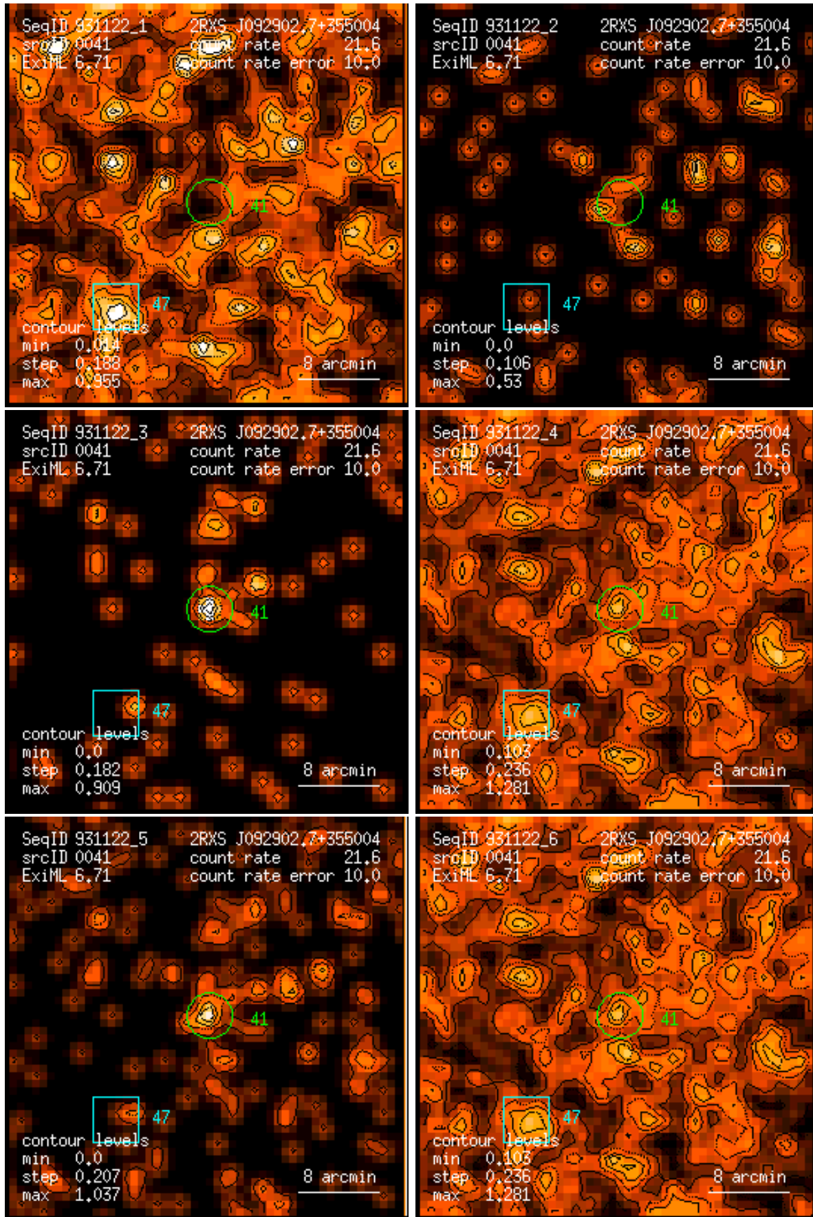
Figure 41: RASS 931122: detection 0041: band rate images, Gaussian filter: (1) PSPC channels 11 – 41, (2) 52 – 90, (3) 91 – 201, (4) 11 – 235, (5) 52 – 201, (6) 11 – 201. Broad band rates in counts/ks. Band rate contour levels in counts/ks/arcmin 2 .
