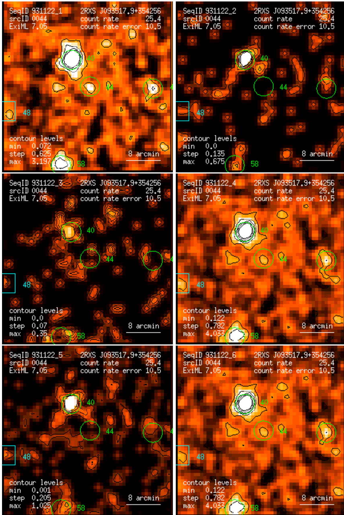
Figure 44: RASS 931122: detection 0044: band rate images, Gaussian filter: (1) PSPC channels 11 – 41, (2) 52 – 90, (3) 91 – 201, (4) 11 – 235, (5) 52 – 201, (6) 11 – 201. Broad band rates in counts/ks. Band rate contour levels in counts/ks/arcmin 2 .
