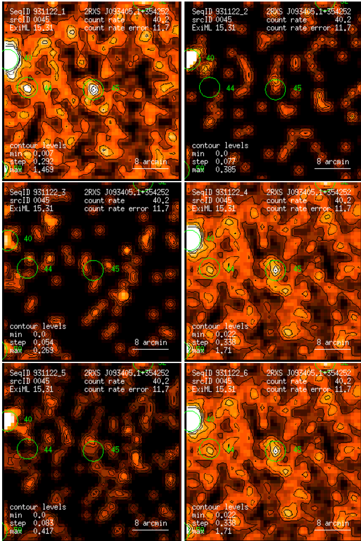
Figure 45: RASS 931122: detection 0045: band rate images, Gaussian filter: (1) PSPC channels 11 – 41, (2) 52 – 90, (3) 91 – 201, (4) 11 – 235, (5) 52 – 201, (6) 11 – 201. Broad band rates in counts/ks. Band rate contour levels in counts/ks/arcmin 2 .
