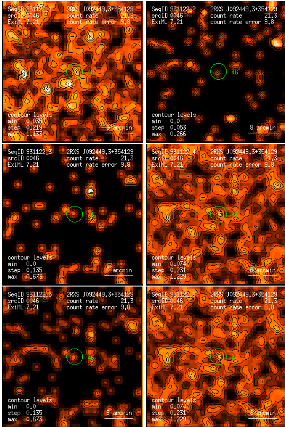
Figure 46: RASS 931122: detection 0046: band rate images, Gaussian filter: (1) PSPC channels 11 – 41, (2) 52 – 90, (3) 91 – 201, (4) 11 – 235, (5) 52 – 201, (6) 11 – 201. Broad band rates in counts/ks. Band rate contour levels in counts/ks/arcmin 2 .
