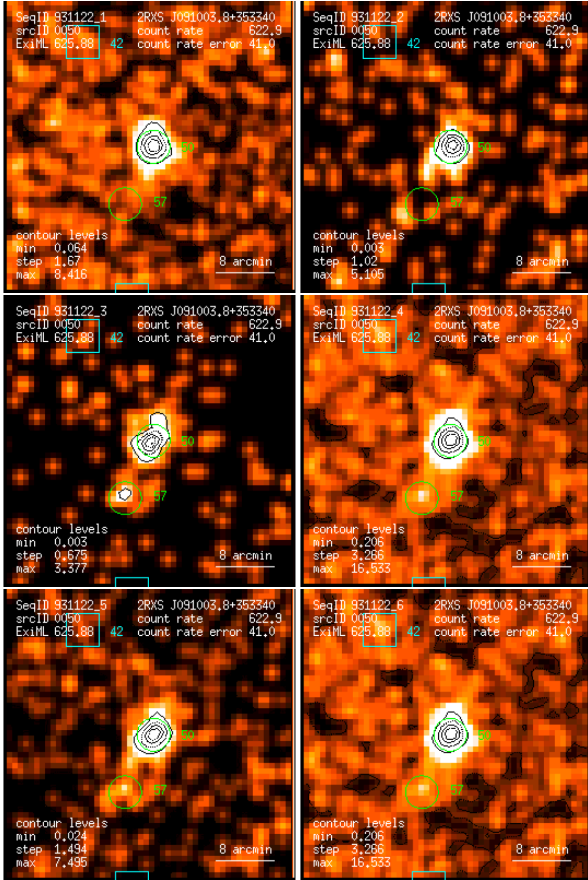
Figure 50: RASS 931122: detection 0050: band rate images, Gaussian filter: (1) PSPC channels 11 – 41, (2) 52 – 90, (3) 91 – 201, (4) 11 – 235, (5) 52 – 201, (6) 11 – 201. Broad band rates in counts/ks. Band rate contour levels in counts/ks/arcmin 2 .
