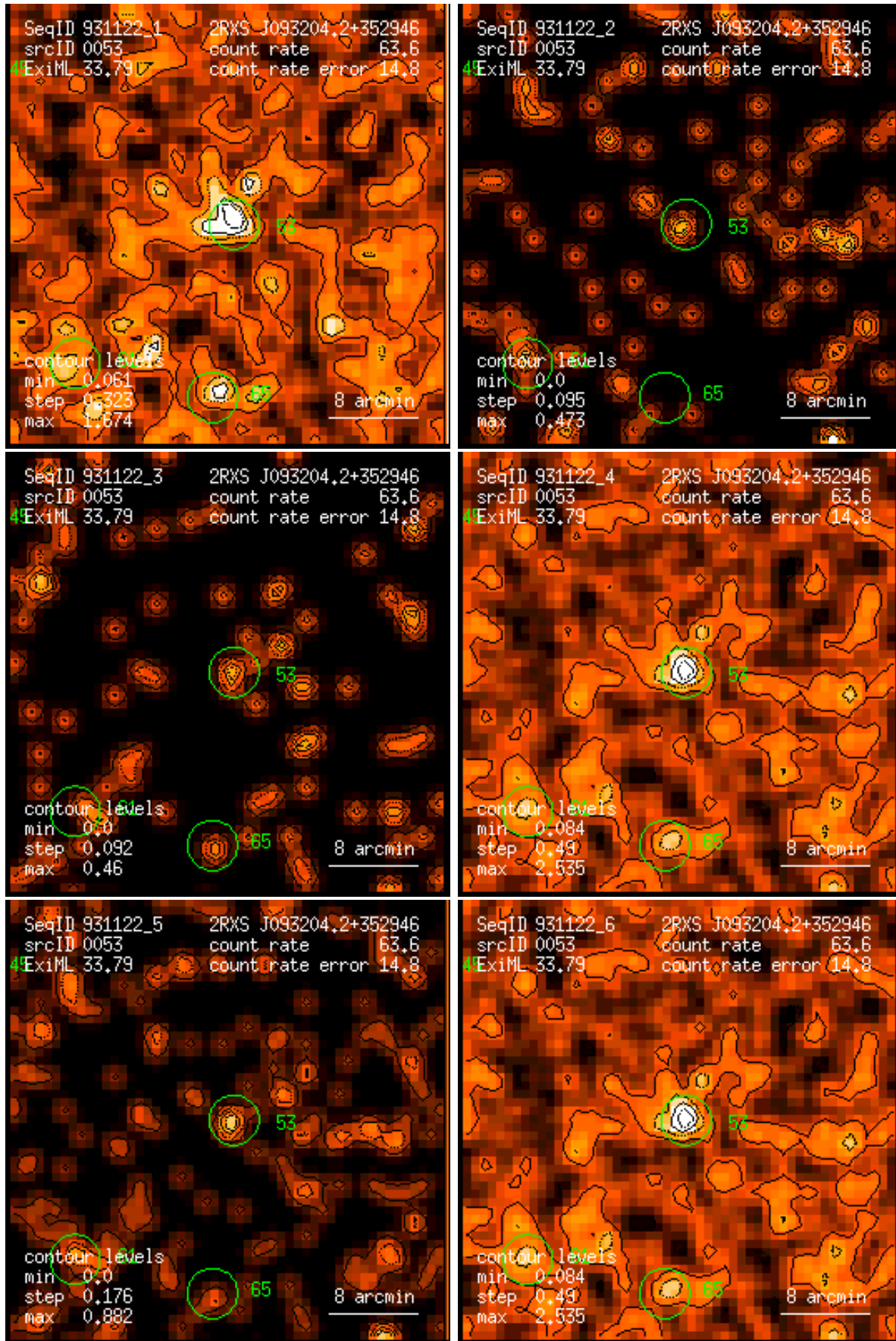
Figure 53: RASS 931122: detection 0053: band rate images, Gaussian filter: (1) PSPC channels 11 – 41, (2) 52 – 90, (3) 91 – 201, (4) 11 – 235, (5) 52 – 201, (6) 11 – 201. Broad band rates in counts/ks. Band rate contour levels in counts/ks/arcmin 2 .
