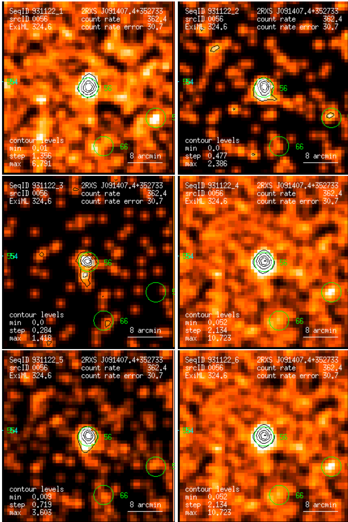
Figure 56: RASS 931122: detection 0056: band rate images, Gaussian filter: (1) PSPC channels 11 – 41, (2) 52 – 90, (3) 91 – 201, (4) 11 – 235, (5) 52 – 201, (6) 11 – 201. Broad band rates in counts/ks. Band rate contour levels in counts/ks/arcmin 2 .
