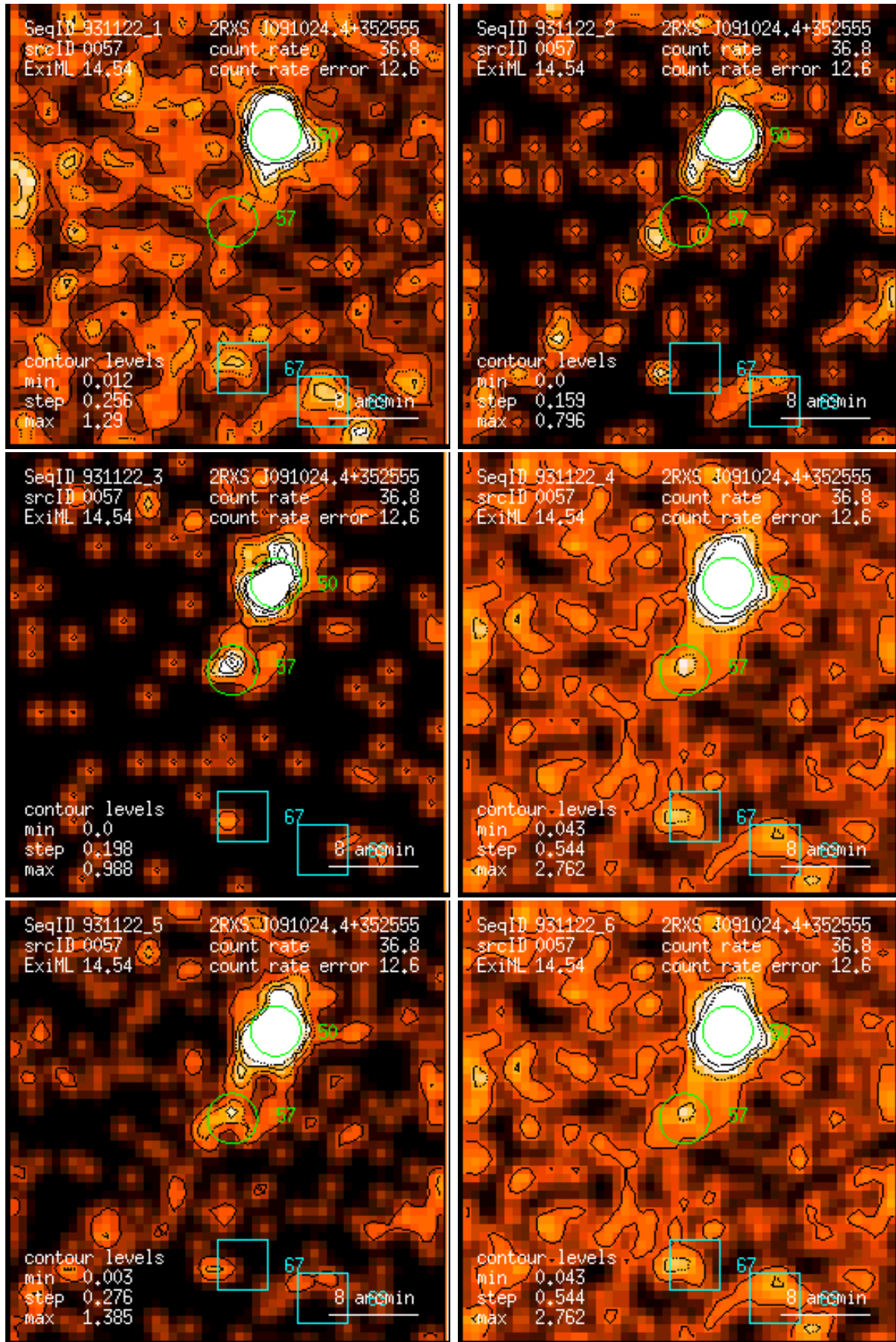
Figure 57: RASS 931122: detection 0057: band rate images, Gaussian filter: (1) PSPC channels 11 – 41, (2) 52 – 90, (3) 91 – 201, (4) 11 – 235, (5) 52 – 201, (6) 11 – 201. Broad band rates in counts/ks. Band rate contour levels in counts/ks/arcmin 2 .
