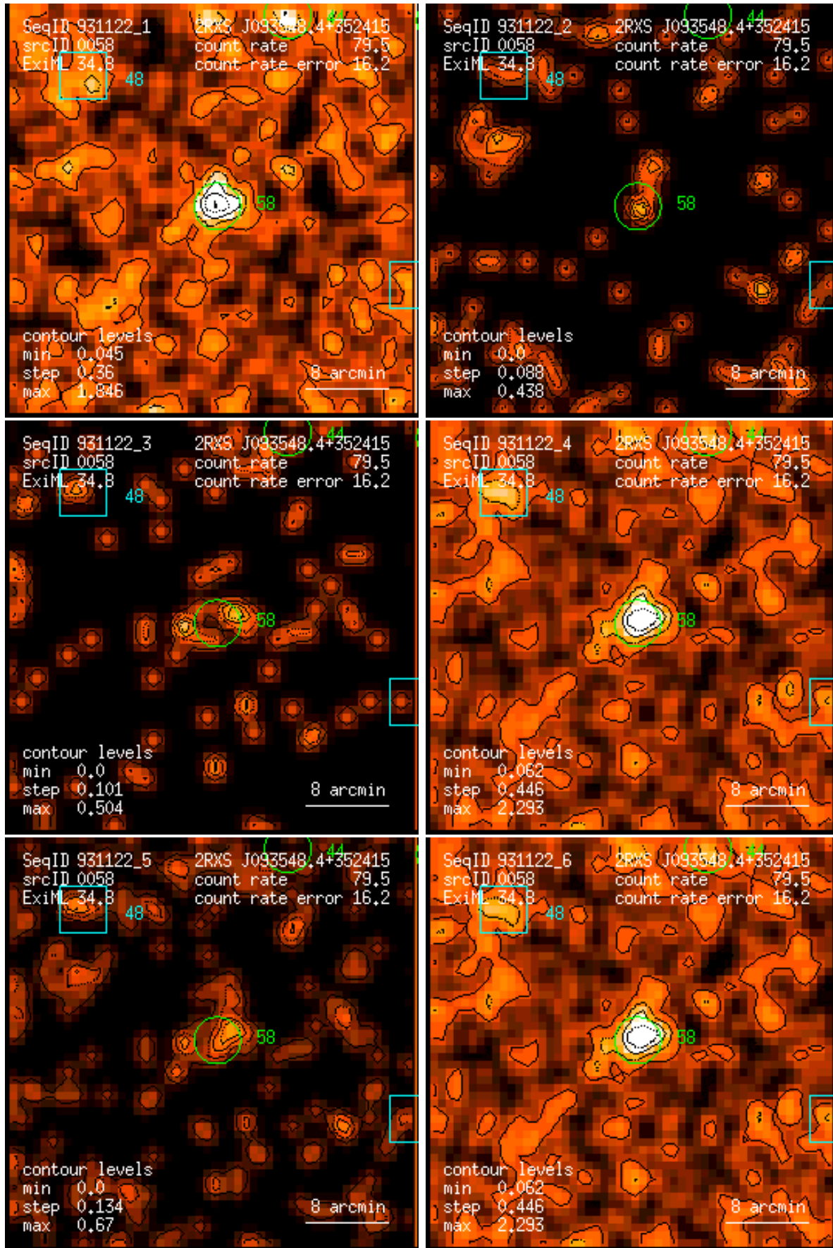
Figure 58: RASS 931122: detection 0058: band rate images, Gaussian filter: (1) PSPC channels 11 – 41, (2) 52 – 90, (3) 91 – 201, (4) 11 – 235, (5) 52 – 201, (6) 11 – 201. Broad band rates in counts/ks. Band rate contour levels in counts/ks/arcmin 2 .
