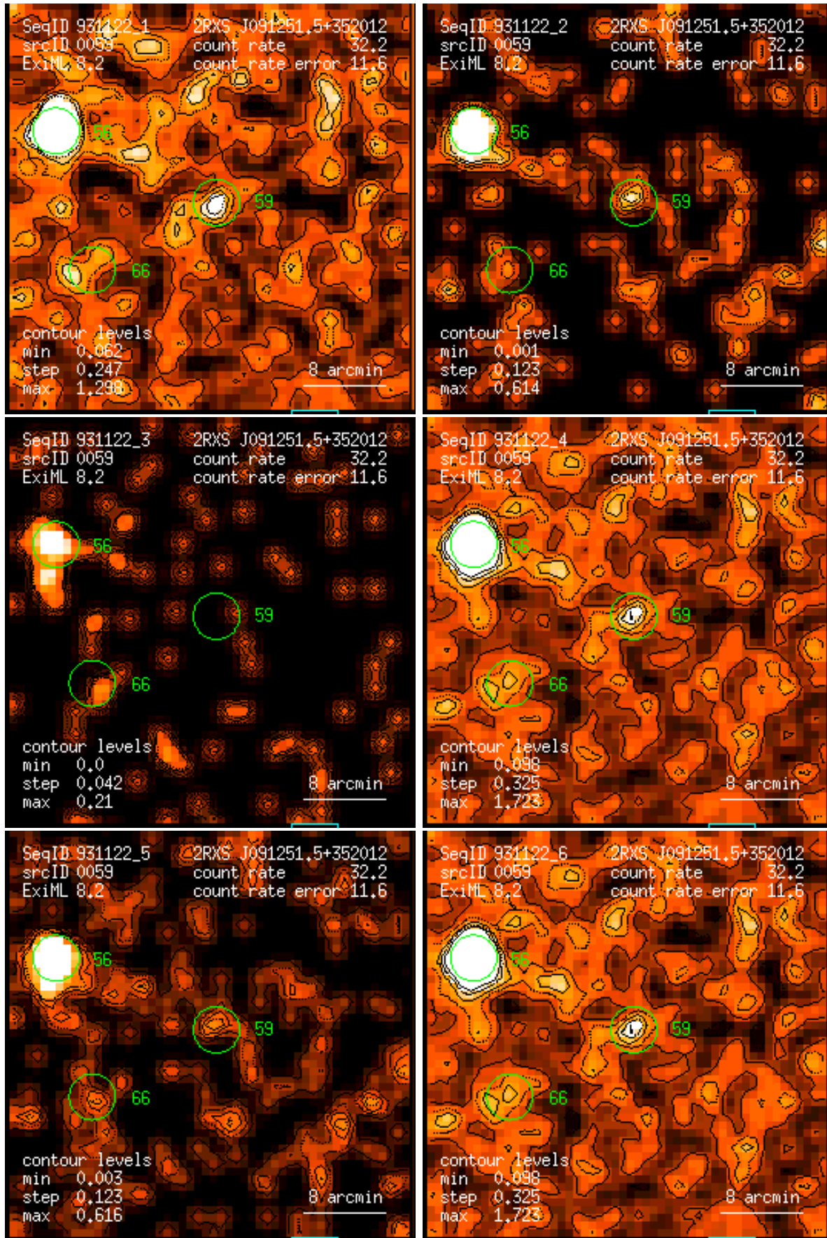
Figure 59: RASS 931122: detection 0059: band rate images, Gaussian filter: (1) PSPC channels 11 – 41, (2) 52 – 90, (3) 91 – 201, (4) 11 – 235, (5) 52 – 201, (6) 11 – 201. Broad band rates in counts/ks. Band rate contour levels in counts/ks/arcmin 2 .
