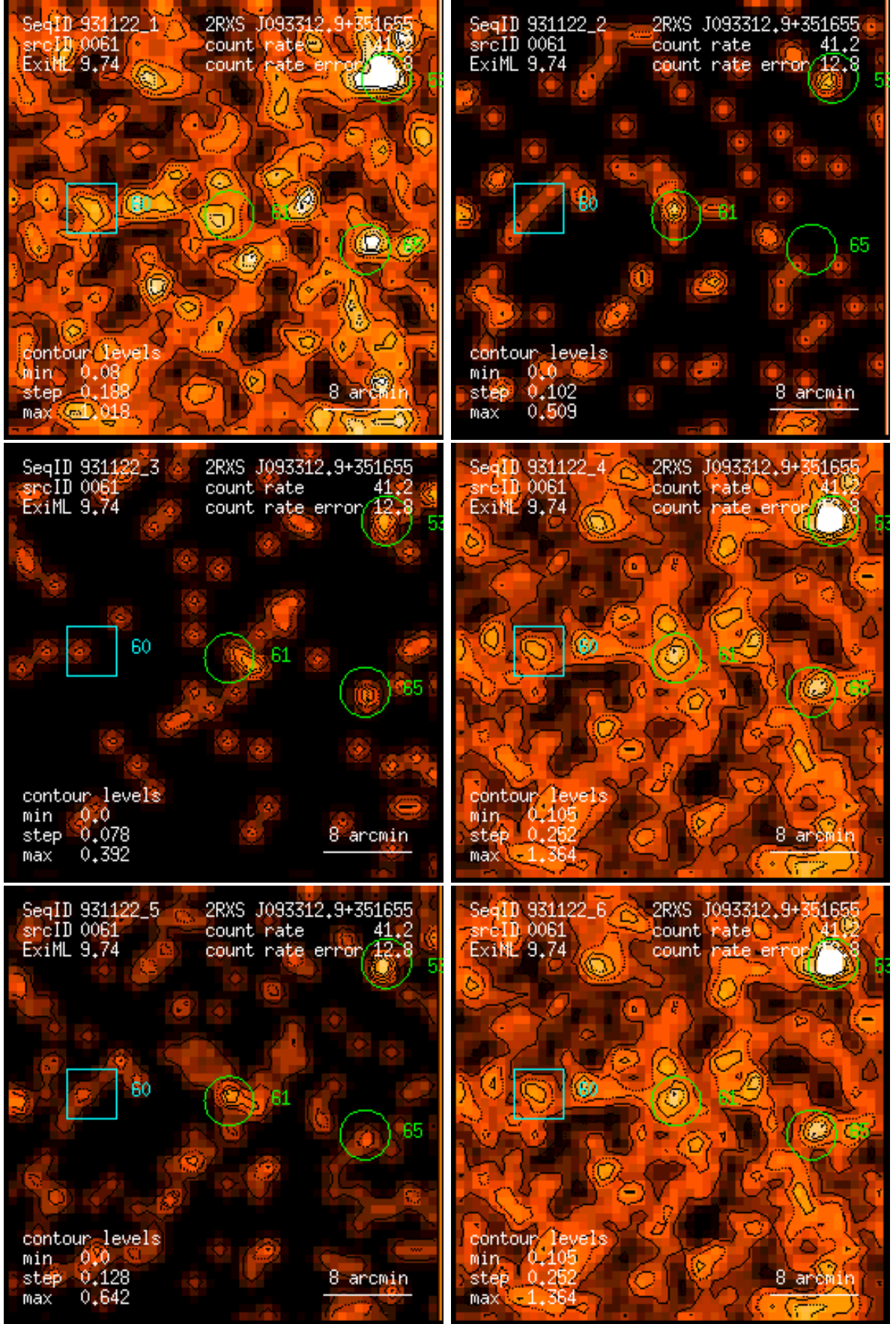
Figure 61: RASS 931122: detection 0061: band rate images, Gaussian filter: (1) PSPC channels 11 – 41, (2) 52 – 90, (3) 91 – 201, (4) 11 – 235, (5) 52 – 201, (6) 11 – 201. Broad band rates in counts/ks. Band rate contour levels in counts/ks/arcmin 2 .
