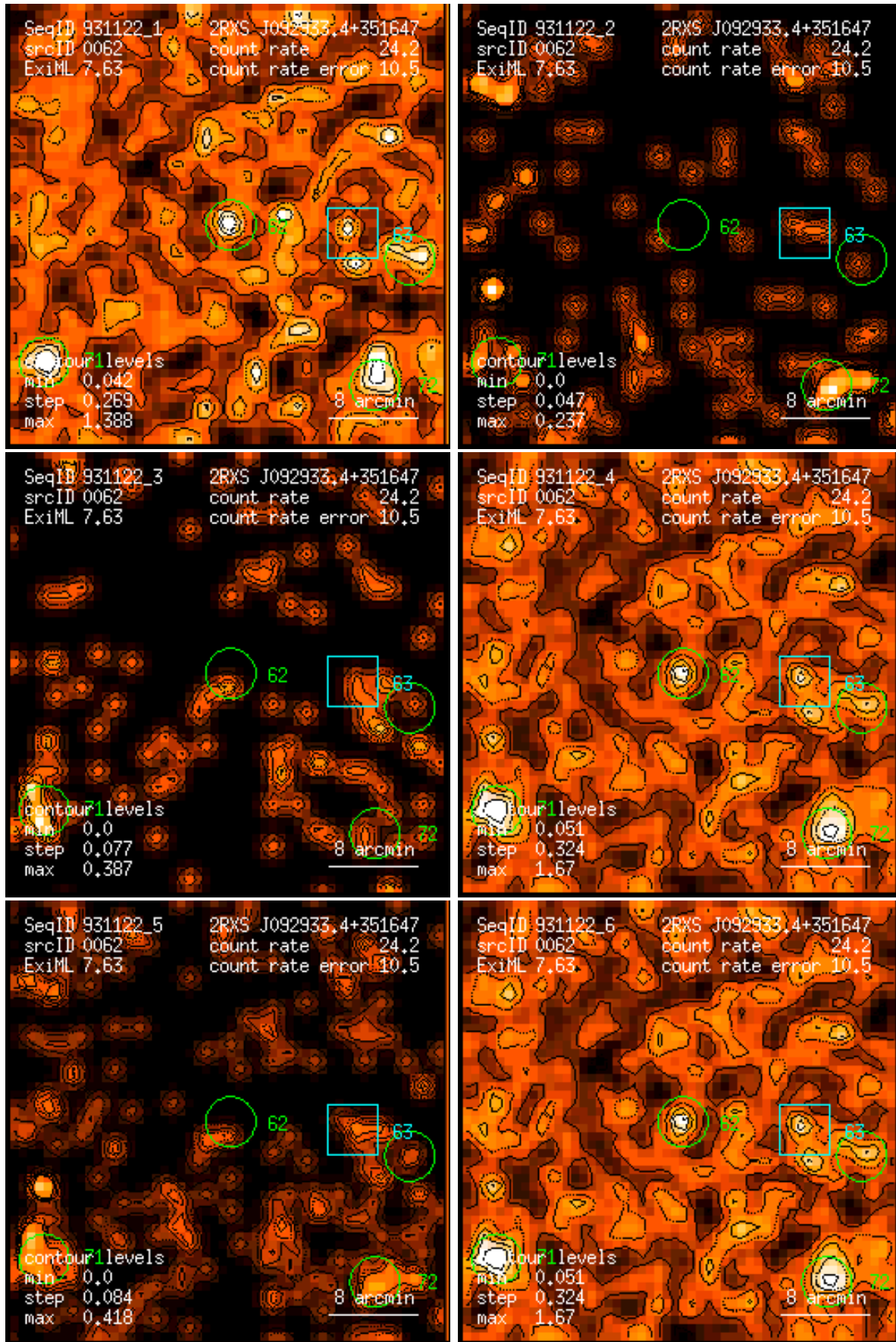
Figure 62: RASS 931122: detection 0062: band rate images, Gaussian filter: (1) PSPC channels 11 – 41, (2) 52 – 90, (3) 91 – 201, (4) 11 – 235, (5) 52 – 201, (6) 11 – 201. Broad band rates in counts/ks. Band rate contour levels in counts/ks/arcmin 2 .
