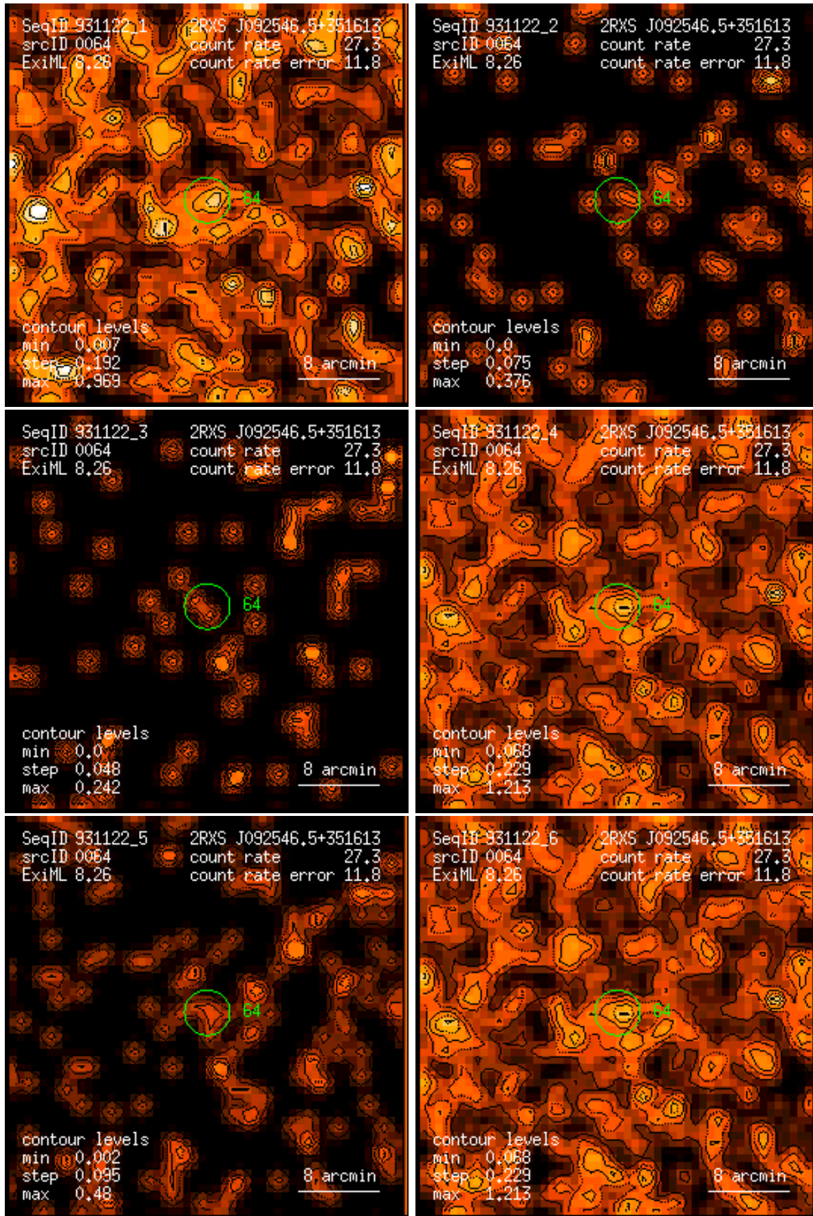
Figure 64: RASS 931122: detection 0064: band rate images, Gaussian filter: (1) PSPC channels 11 – 41, (2) 52 – 90, (3) 91 – 201, (4) 11 – 235, (5) 52 – 201, (6) 11 – 201. Broad band rates in counts/ks. Band rate contour levels in counts/ks/arcmin 2 .
