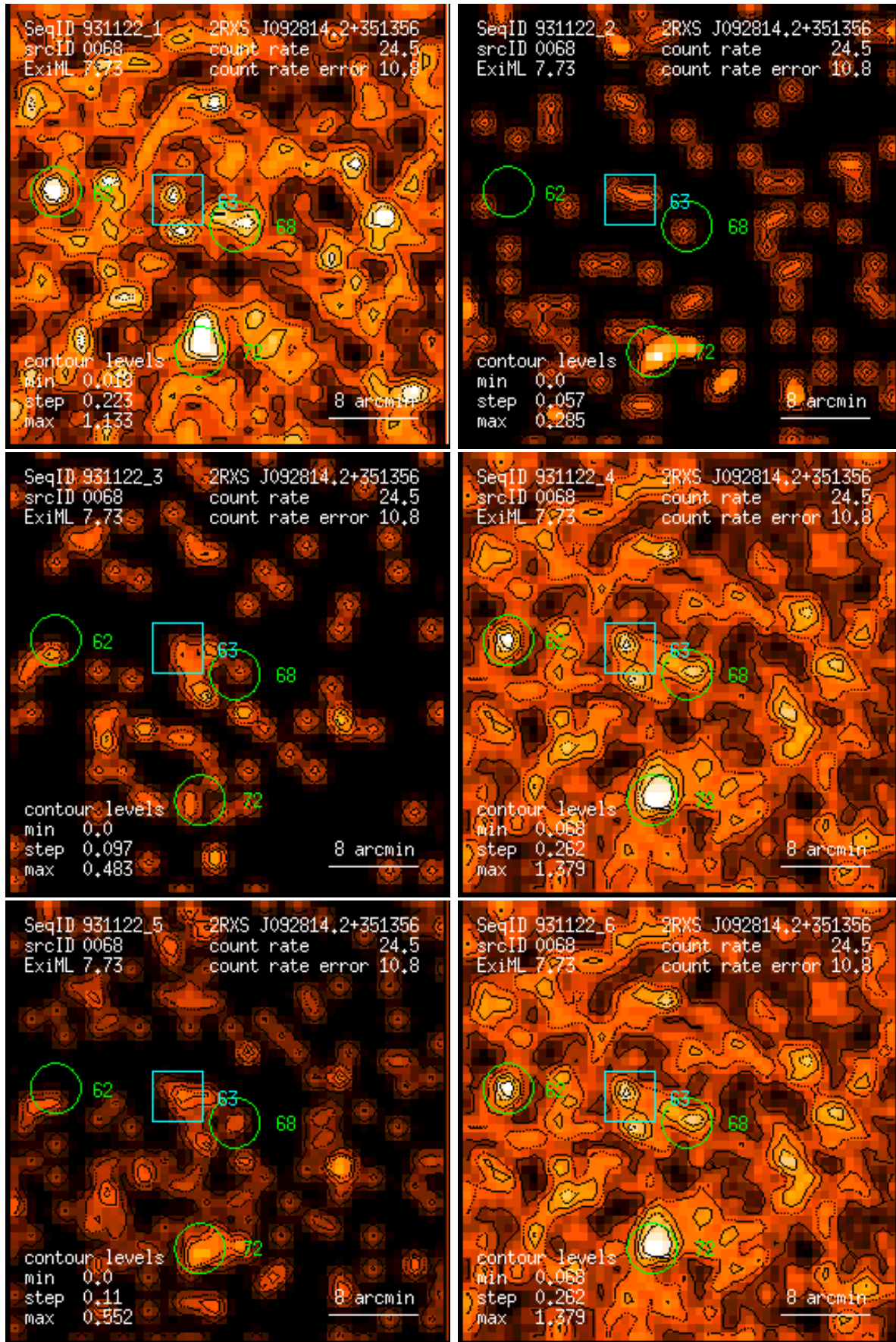
Figure 68: RASS 931122: detection 0068: band rate images, Gaussian filter: (1) PSPC channels 11 – 41, (2) 52 – 90, (3) 91 – 201, (4) 11 – 235, (5) 52 – 201, (6) 11 – 201. Broad band rates in counts/ks. Band rate contour levels in counts/ks/arcmin 2 .
