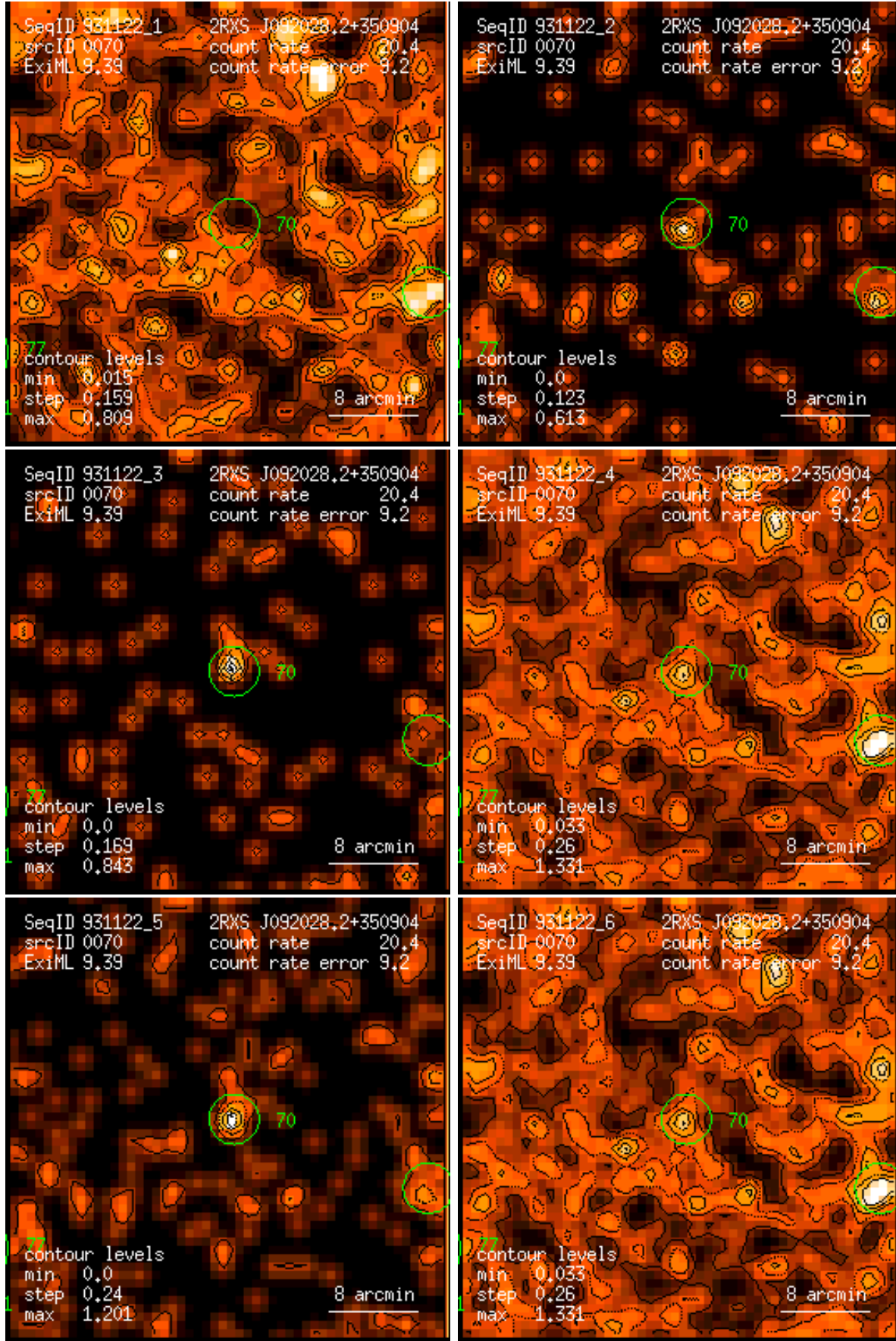
Figure 70: RASS 931122: detection 0070: band rate images, Gaussian filter: (1) PSPC channels 11 – 41, (2) 52 – 90, (3) 91 – 201, (4) 11 – 235, (5) 52 – 201, (6) 11 – 201. Broad band rates in counts/ks. Band rate contour levels in counts/ks/arcmin 2 .
